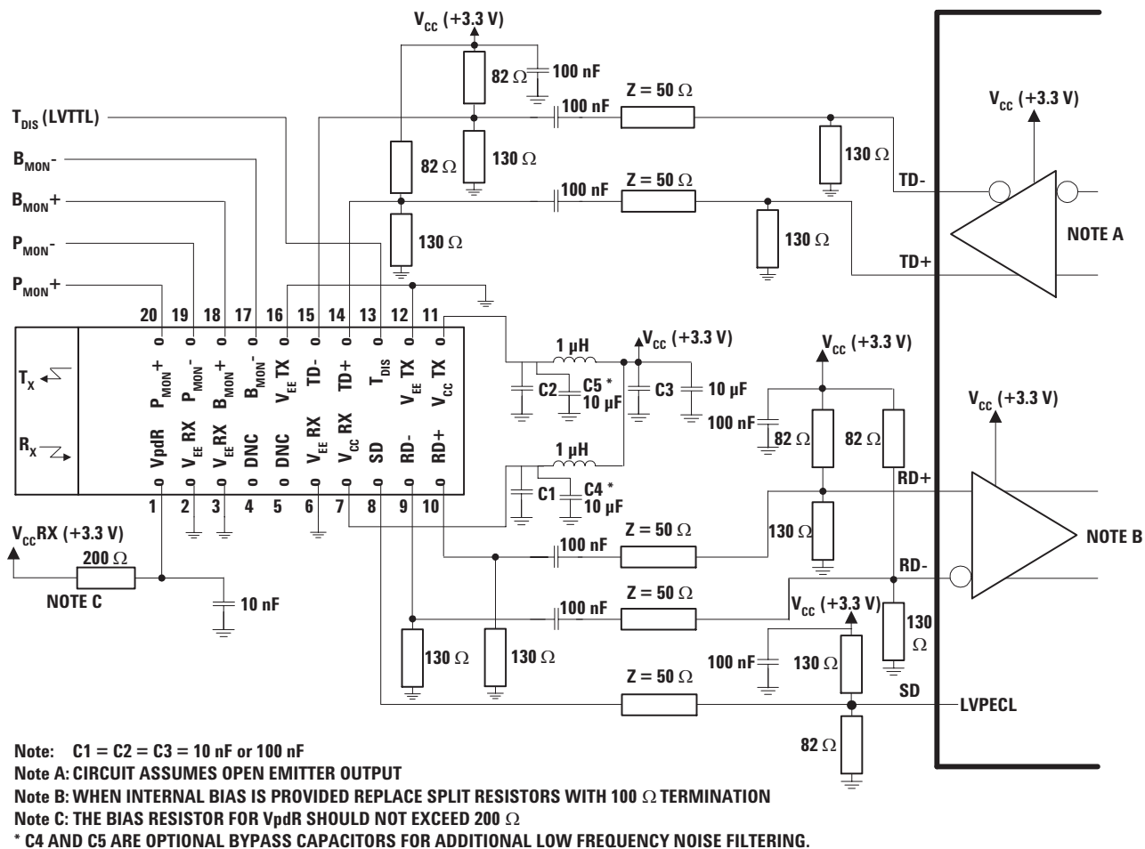
Figure 6b. Recommended ac coupled interface circuit
