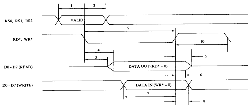
Figure 7. MPU Read/Write Timing Dimensions.
