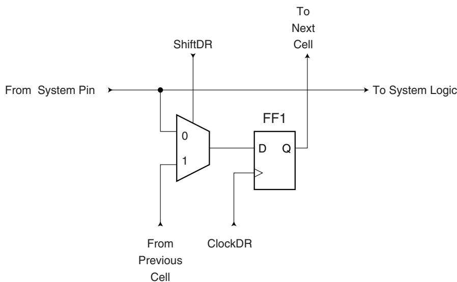
Figure 24-6. Observe-only Cell
