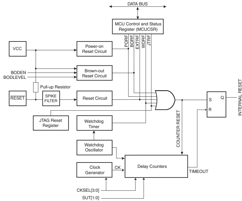
Figure 10-1. Reset Logic
