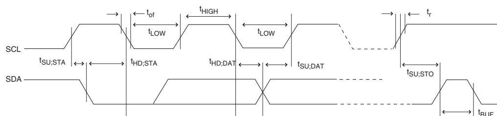
Figure 27-4. Two-wire Serial Bus Timing
