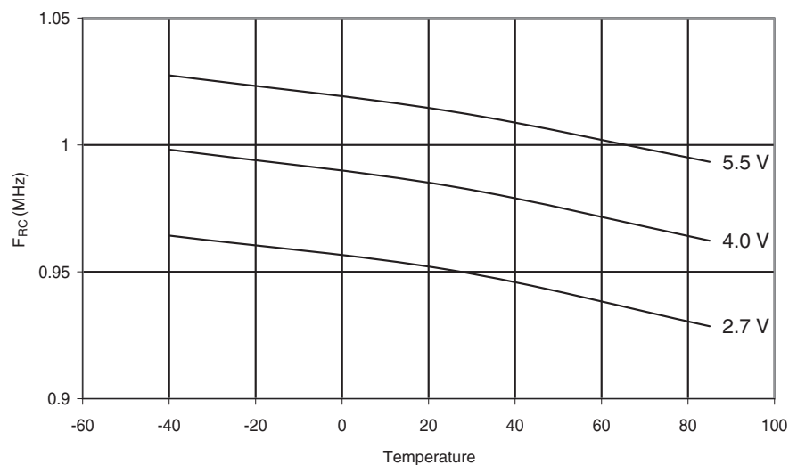
Figure 28-47. Calibrated 1 MHz RC Oscillator Frequency vs. V_{CC}
