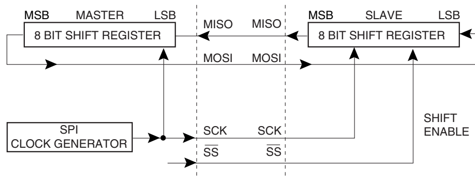
Figure 18-1. SPI Master-Slave Interconnection
