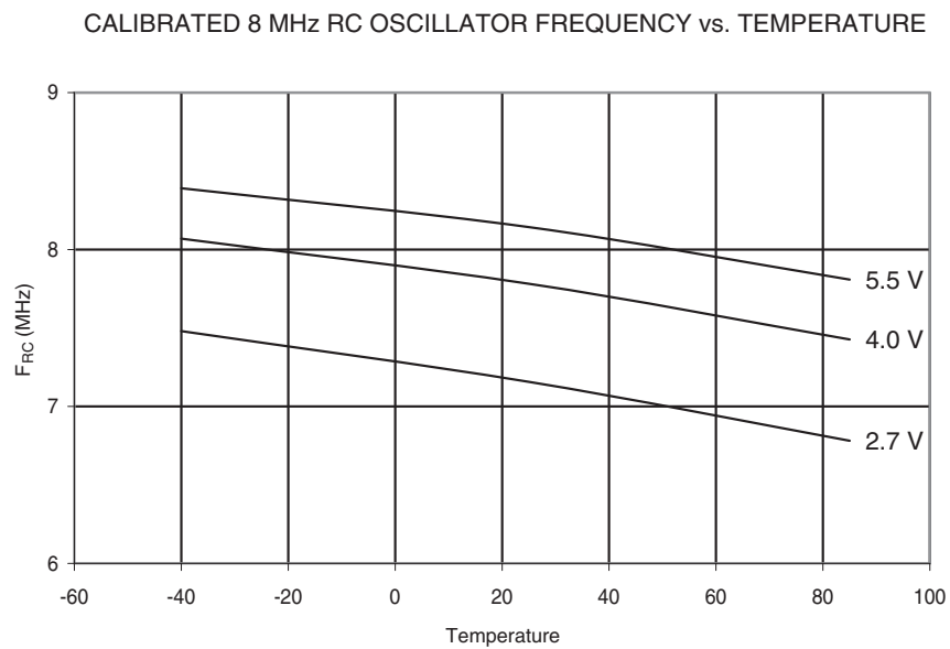
Figure 28-37. Calibrated 8 MHz RC Oscillator Frequency vs. Temperature
