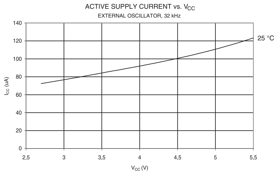
Figure 28-7. Active Supply Current vs. V_{CC} (32 kHz External Oscillator)
