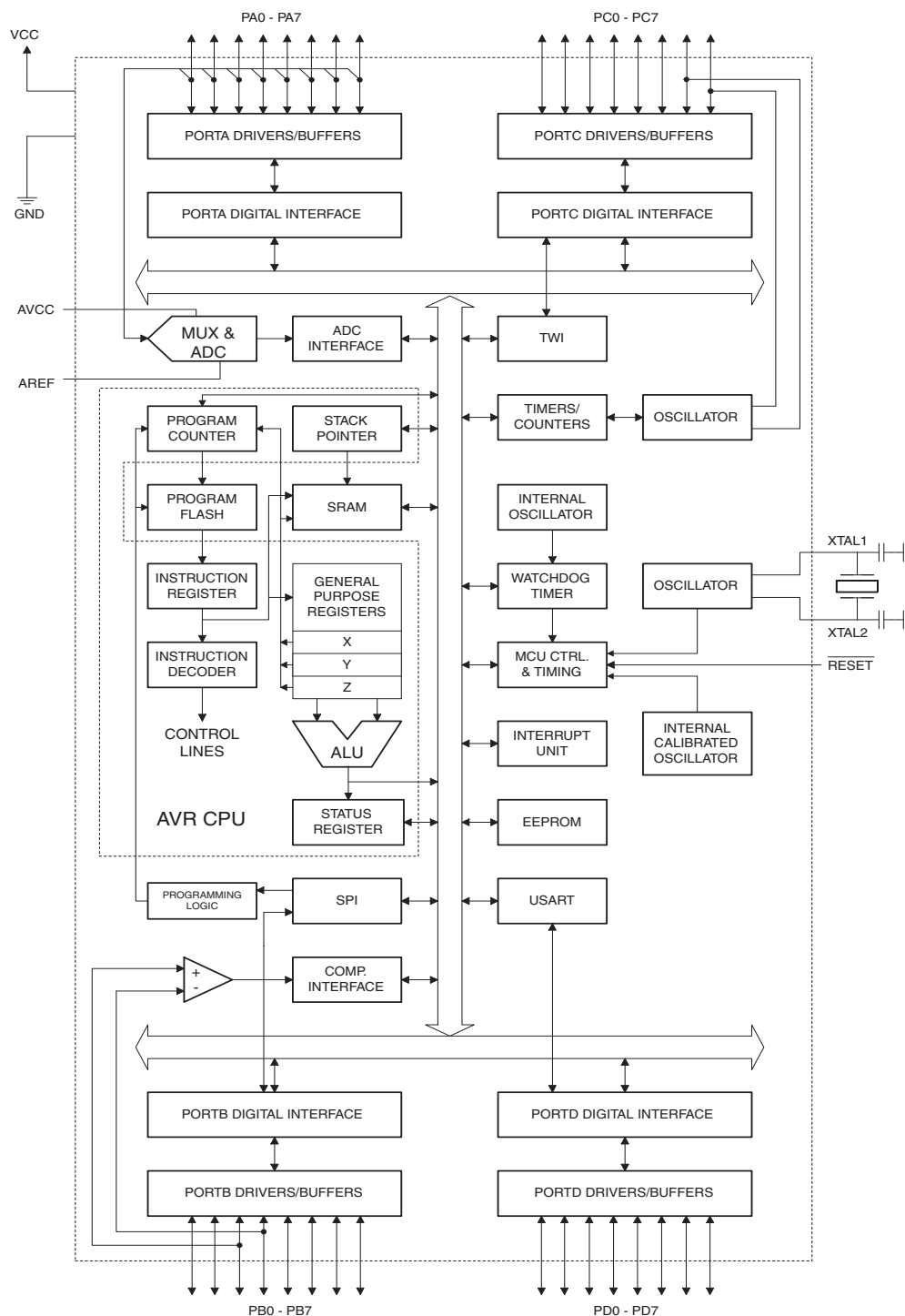
Figure 2-1. Block Diagram
