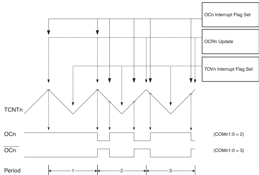
Figure 14-7. Phase Correct PWM Mode, Timing Diagram
