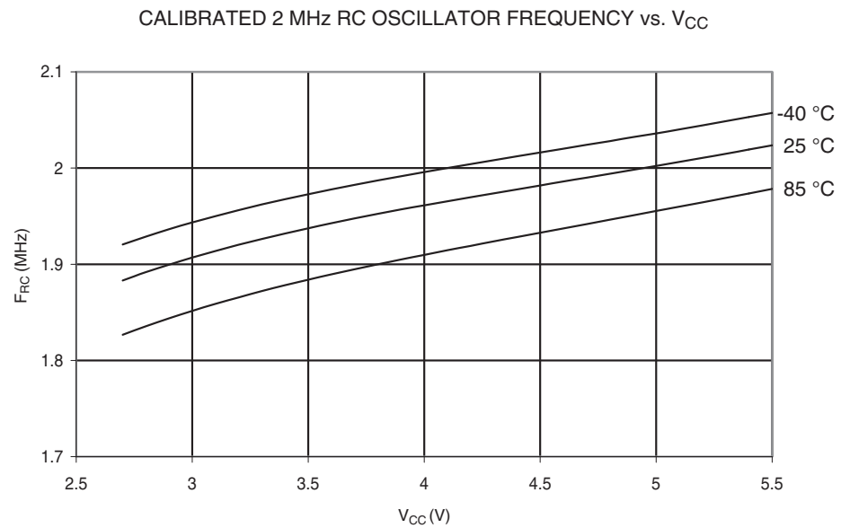
Figure 28-44. Calibrated 2 MHz RC Oscillator Frequency vs. V_{CC}
