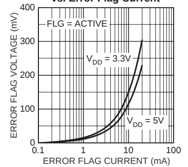
Error Flag Voltage vs. Error Flag Current
