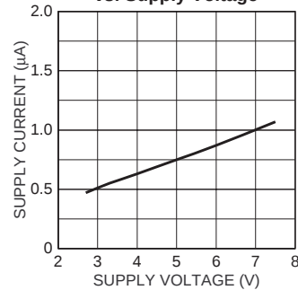
Off-State Supply Current vs. Supply Voltage
