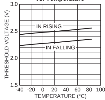
UVLO Threshold Voltage vs. Temperature
