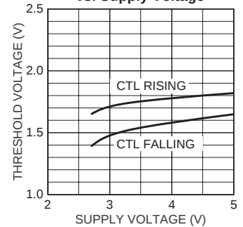
Control Threshold vs. Supply Voltage
