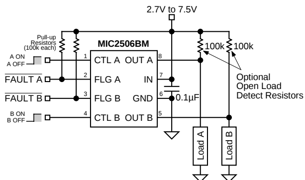
Single and Dual Switch/Circuit Breakers with Open-Load Detection and Fault Output
