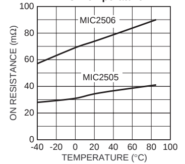
Output On Resistance vs. Temperature
