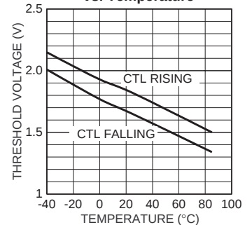
Control Threshold vs. Temperature
