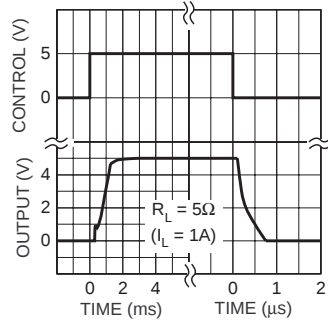
MIC2506 Turn-On, Turn-Off Characteristics
