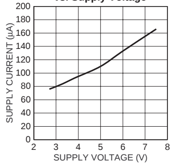
On-State Supply Current vs. Supply Voltage
