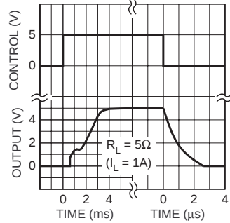
MIC2505 Turn-On, Turn-Off Characteristics
