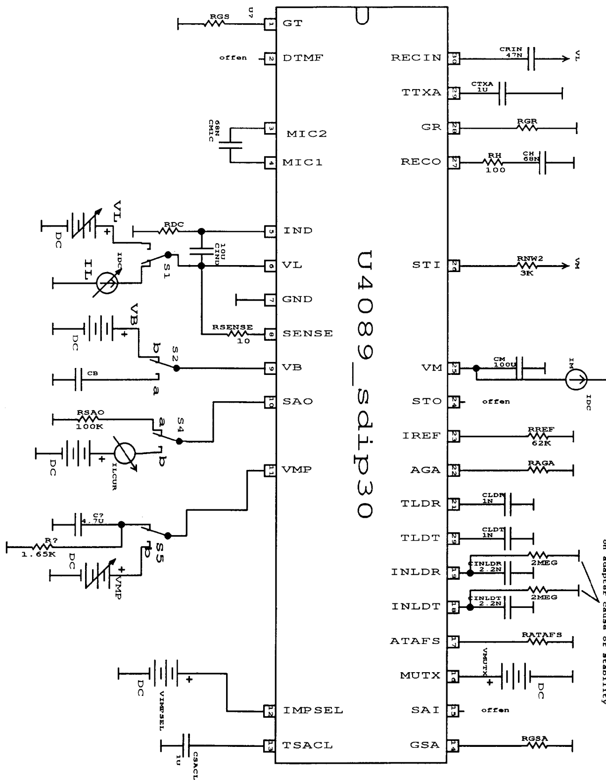
Figure 22. DC ramps
