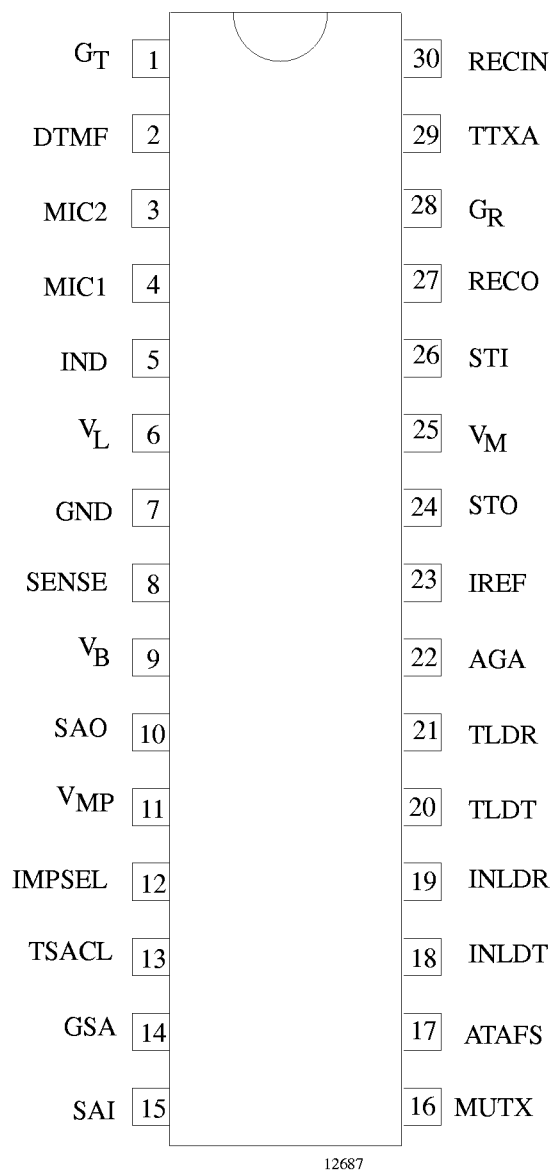
Figure 3. Pinning SDIP30
