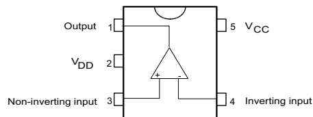
TS941ID-TS941IDT
