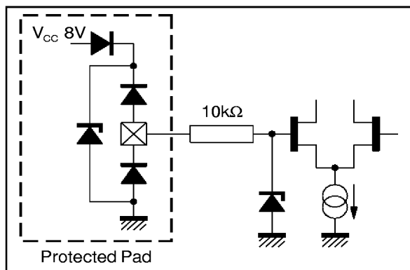
Figure 12 : I^2C Bus (SCL) (Pin 21)
