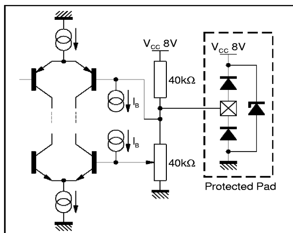
Figure 9 : Input Fast Blanking (Pins 18, 19)
