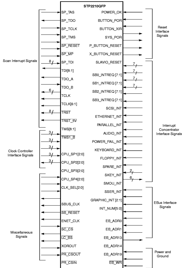
Figure 2. STP2210QFP Logical Connections
