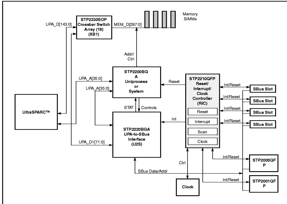
Figure 3. STP2210QFP Typical Application Diagram
