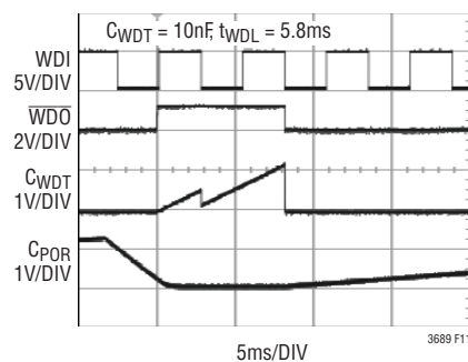
Figure 11. Window Watchdog Waveforms ( \overline{\text{W/T}} = Low)
