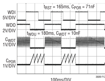
Figure 12. Timeout Watchdog Waveforms ( \overline{\text{W/T}} = High)
