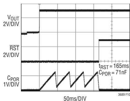
Figure 10. Reset Timer Waveforms
