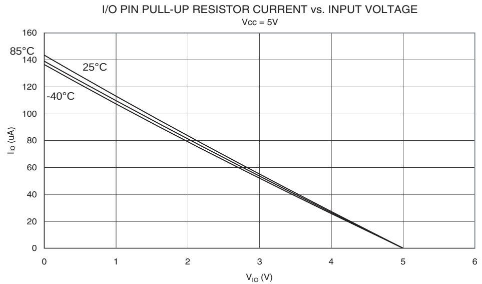
Figure 156. I/O Pin Pull-up Resistor Current vs. Input Voltage ( V_{CC} = 5V )
