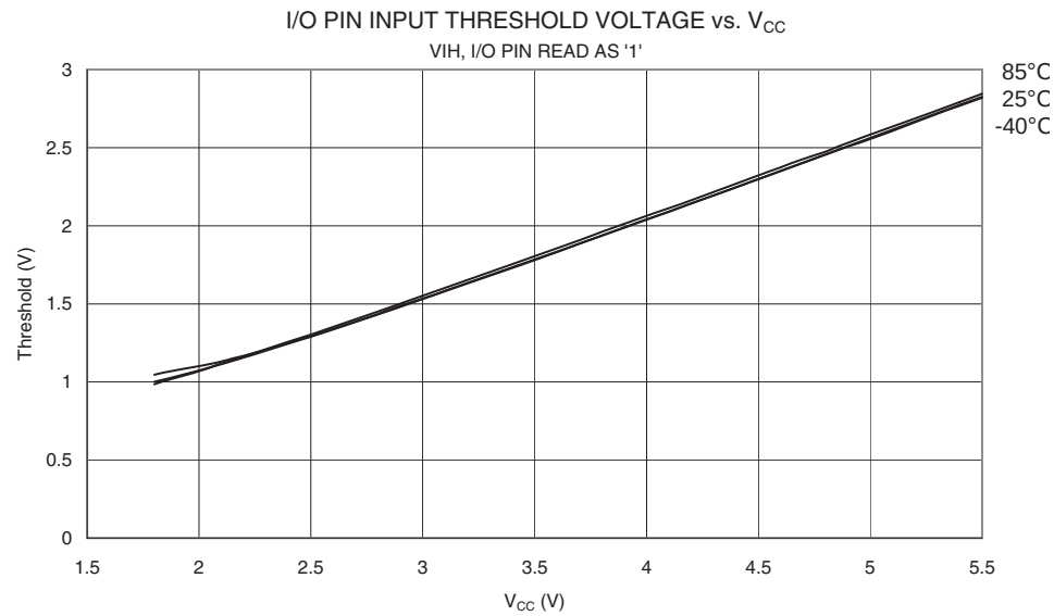
Pin Thresholds and hysteresis Figure 174. I/O Pin Input Threshold Voltage vs. V_{CC} ( V_{IH} , I/O Pin Read as “1”)
