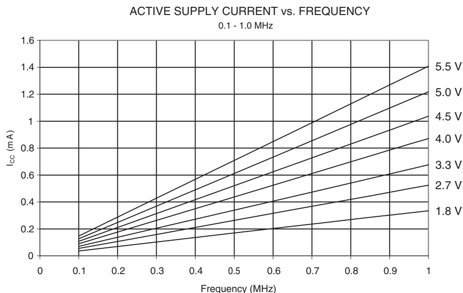
Figure 142. Active Supply Current vs. Frequency (0.1 - 1.0 MHz)
