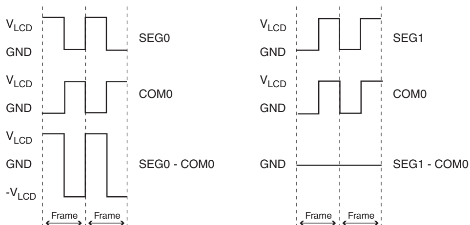
Figure 100. Driving a LCD with One Common Terminal
