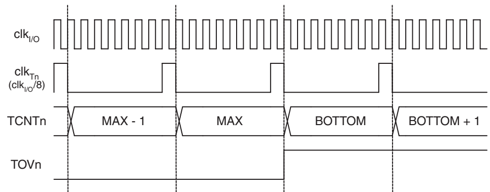
Figure 62. Timer/Counter Timing Diagram, with Prescaler ( f_{\text{clk\_I/O}}/8 )
