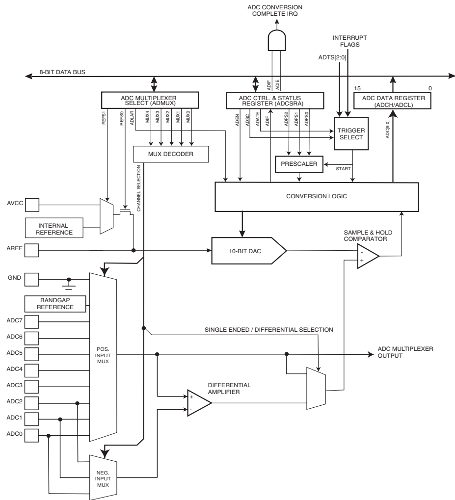
ADC CONVERSION
