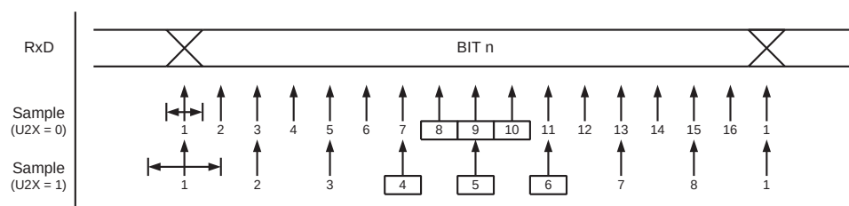
Figure 75. Sampling of Data and Parity Bit
