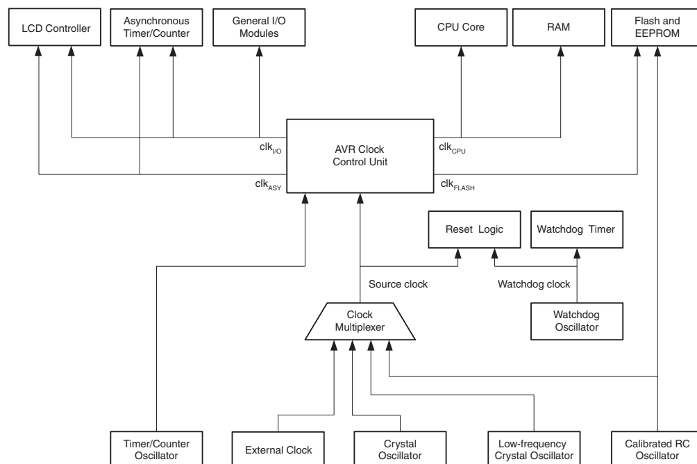
Figure 12. Clock Distribution
