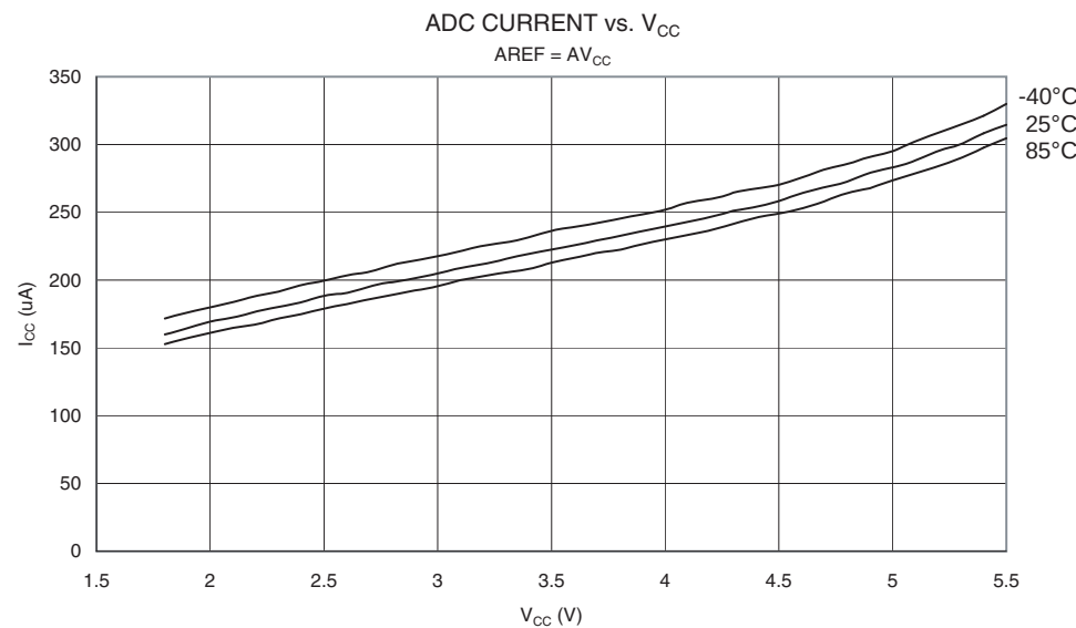
Figure 191. ADC Current vs. V_{CC} (AREF = AVCC)
