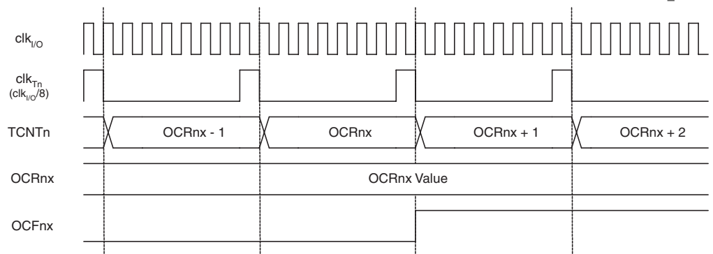
Figure 37. Timer/Counter Timing Diagram, Setting of OCF0A, with Prescaler ( f_{\text{clk\_I/O}}/8 )
