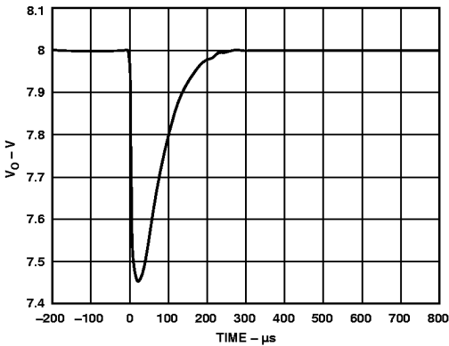
Figure 20. Predicted Response for 24 A Step Load Change in Load Current, di/dt = 12\text{ A}/\mu s , for C_{LOAD} = 500\text{ }\mu F and R_{ESR} = 20\text{ m}\Omega
