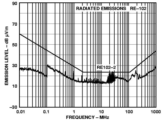
Figure 14. Radiated Emissions, MIL-STD-461D, RE102, Vertical Polarity, 100 W Load
