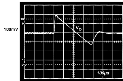
Figure 28. Output Voltage Transient Response to a 25 A to 1 A Step Change in Load, di/dt = 12 \text{ A}/\mu\text{s} , with 1,000 \mu\text{F} Load Capacitance ( R_{\text{ESR}} = 10 \text{ m}\Omega )
