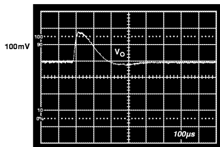
Figure 26. Output Voltage Transient Response to a 25 A to 4 A Step Change in Load, di/dt = 12 \text{ A}/\mu\text{s} , with 1,000 \mu\text{F} Load Capacitance ( R_{\text{ESR}} = 10 \text{ m}\Omega )
