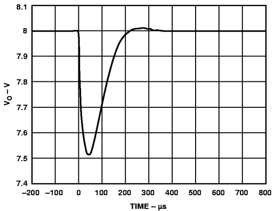
Figure 18. Predicted Response to 24 A Step Change in Load Current, di/dt = 12\text{ A}/\mu s , for C_{LOAD} = 1,000\text{ }\mu F and R_{ESR} = 10\text{ m}\Omega
