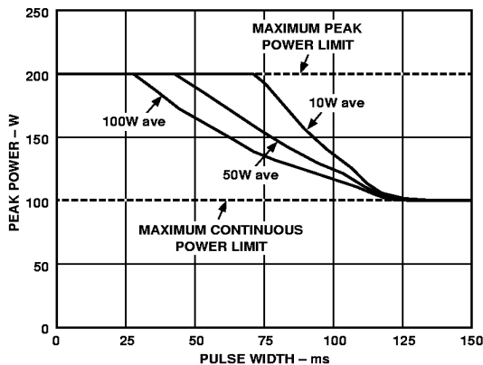
Figure 17. Largest On-State Power vs. Pulse Width that Maintains T_{JMAX} \leq 110^{\circ}C at 90^{\circ}C Baseplate
