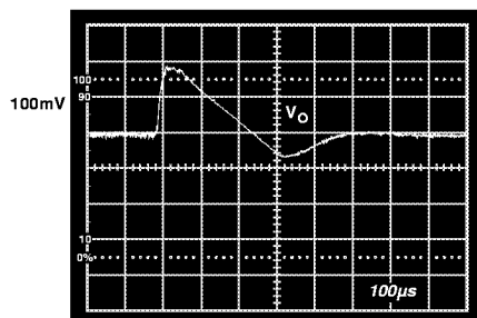
Figure 27. Output Voltage Transient Response to a 25 A to 2 A Step Change in Load, di/dt = 12 \text{ A}/\mu\text{s} , with 1,000 \mu\text{F} Load Capacitance ( R_{\text{ESR}} = 10 \text{ m}\Omega )
