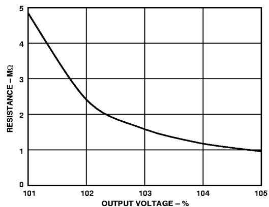
Figure 31. External Resistor for Increasing Output Voltage
