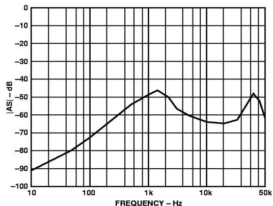
Figure 7. Audio Susceptibility (Magnitude of V_{OUT}/V_{IN} )
