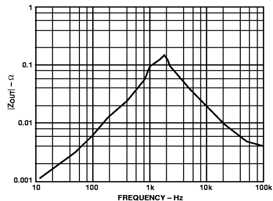
Figure 9. Incremental Output Impedance (Magnitude)
