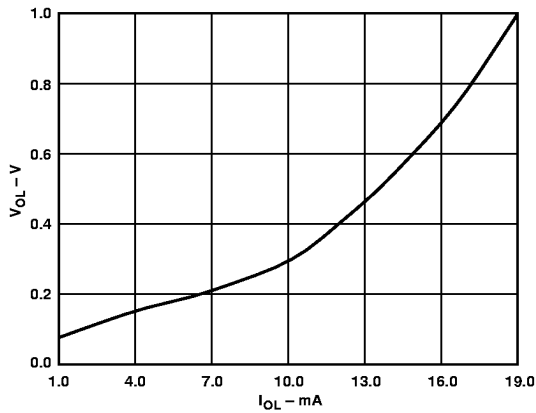
Figure 33. Sink Capability of Status Output
