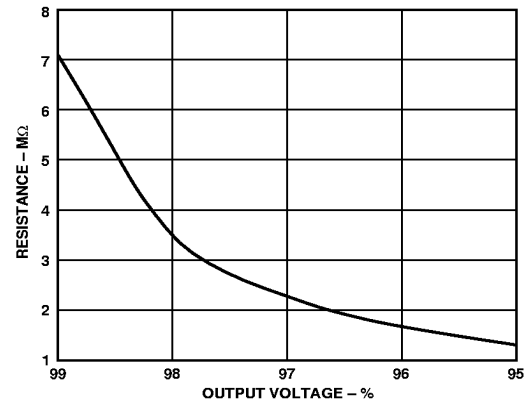
Figure 30. External Resistor Value for Reducing Output Voltage
