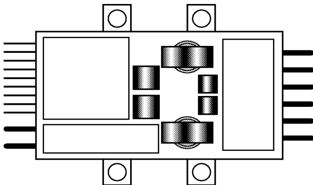
Figure 42. Hot Spots (Shaded Areas) of DC/DC Converter
