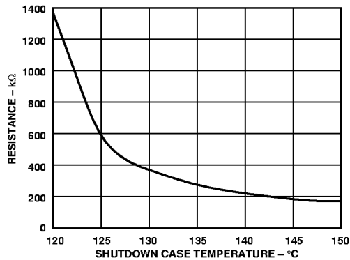
Figure 36. External Resistor Value for Raising Temperature Shutdown Point
