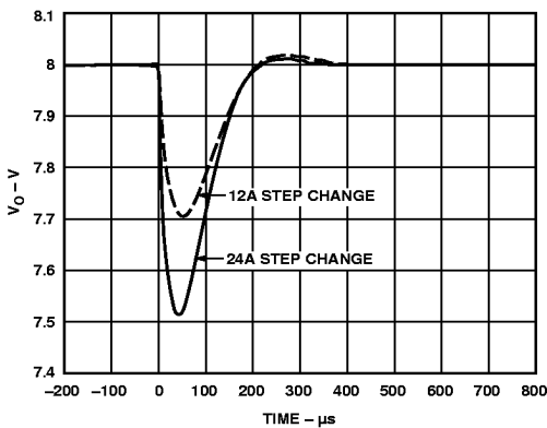
Figure 19. Predicted Response to 12 A and 24 A Step Change in Load Current, di/dt = 12\text{ A}/\mu s , for C_{LOAD} = 1000\text{ }\mu F and R_{ESR} = 10\text{ m}\Omega
