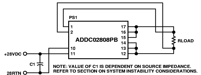
Figure 44. Typical Power Connections and External Parts for Converter
