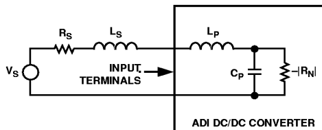
Figure 37. Model of Power Source and POL Converter Connection
