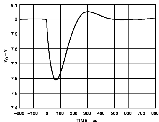
Figure 21. Predicted Response for 24 A Step Load Change in Load Current, di/dt = 12 \text{ A}/\mu\text{s} , for C_{\text{LOAD}} = 2,000 \mu\text{F} and R_{\text{ESR}} = 5 \text{ m}\Omega
