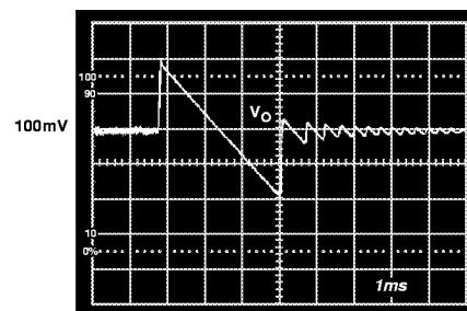
Figure 29. Output Voltage Transient Response to a 25 A to 0.1 A Step Change in Load, di/dt = 12 \text{ A}/\mu\text{s} , with 1,000 \mu\text{F} Load Capacitance ( R_{\text{ESR}} = 10 \text{ m}\Omega )
