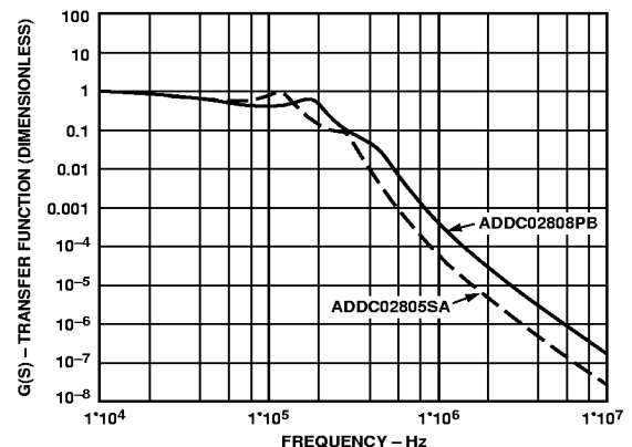
Figure 38. Comparison of Transfer Functions for the Input EMI Filters in ADDC02805SA and ADDC02808PB
