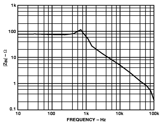
Figure 8. Incremental Input Impedance (Magnitude)
