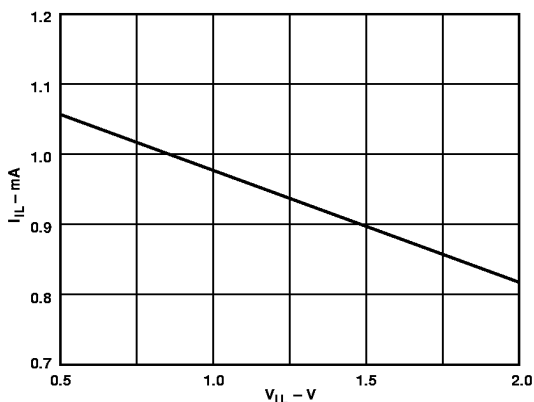
Figure 35. Input Characteristics of Pin 6 When Pulled Low
