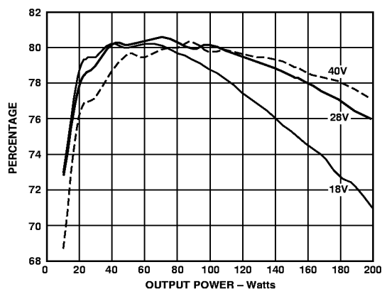
Figure 1. Efficiency vs. Line and Load at +25°C (Load Pulse Width of 50 ms)
