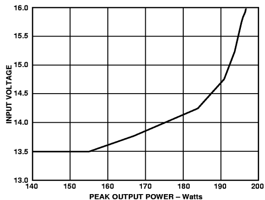
Figure 3. Low Line Dropout vs. Load at 90°C Case Temperature (Load Pulse Width of 50 ms)
