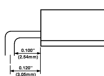
Figure 43. Minimum Bend Radius of 40 Mil (1.02 mm) Pins
