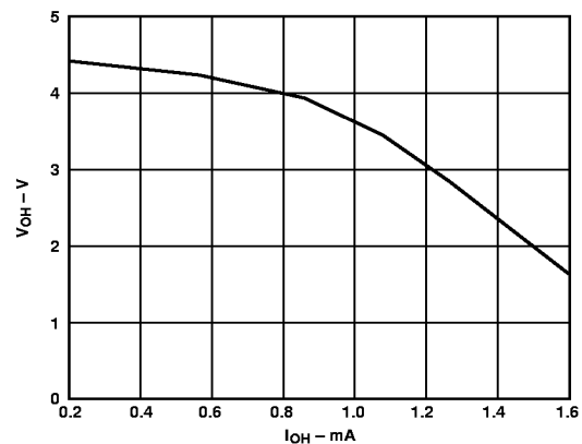
Figure 32. Source Capability of Status Output
