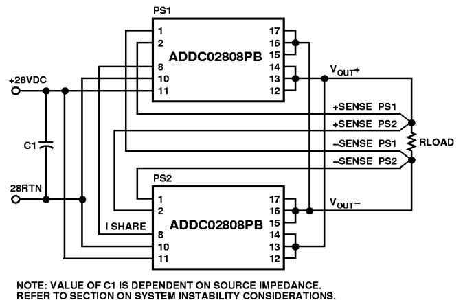
Figure 45. Typical Connections for Paralleling Two Converters
