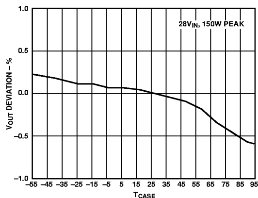
Figure 4. Output Voltage vs. Case Temperature (°C)
