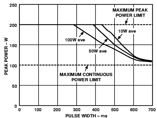
Figure 16. Largest On-State Power vs. Pulse Width that Maintains T_{JMAX} \leq 110^\circ\text{C} at 25^\circ\text{C} Baseplate
