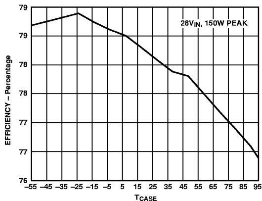
Figure 2. Efficiency vs. Case Temperature (°C) (at Nominal V_{IN} , 75% Max Load, Load Pulse Width of 50 ms)
