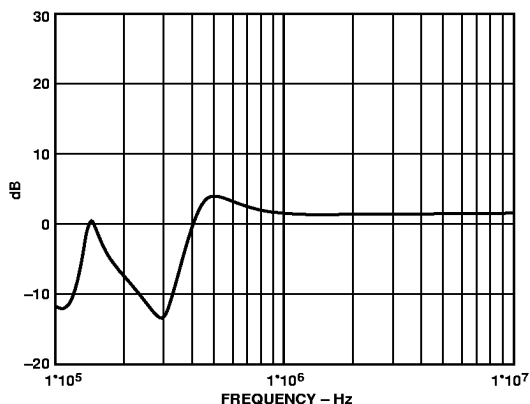
Figure 40. Change in ADDC02808PB Differential Emissions vs. the ADDC02805SA Emissions with External 30 \mu F Capacitor
