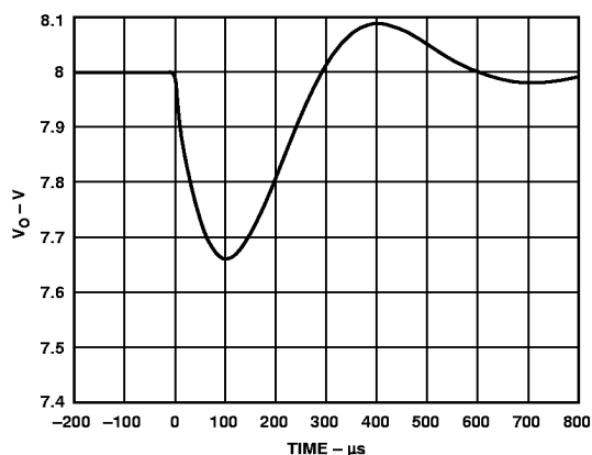
Figure 22. Predicted Response for 24 A Step Load Change in Load Current, di/dt = 12 \text{ A}/\mu\text{s} , for C_{\text{LOAD}} = 4,000 \mu\text{F} and R_{\text{ESR}} = 2.5 \text{ m}\Omega
