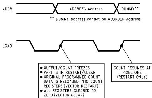
FIGURE 3. ADDRDEC Timing
