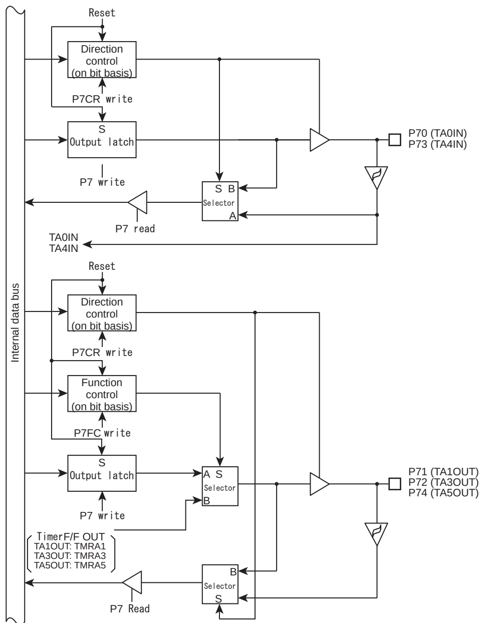
Figure 4-13 Port 70 to 74
