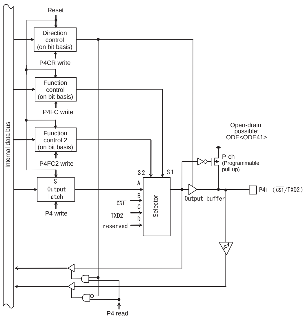
Figure 4-7 Port 41
