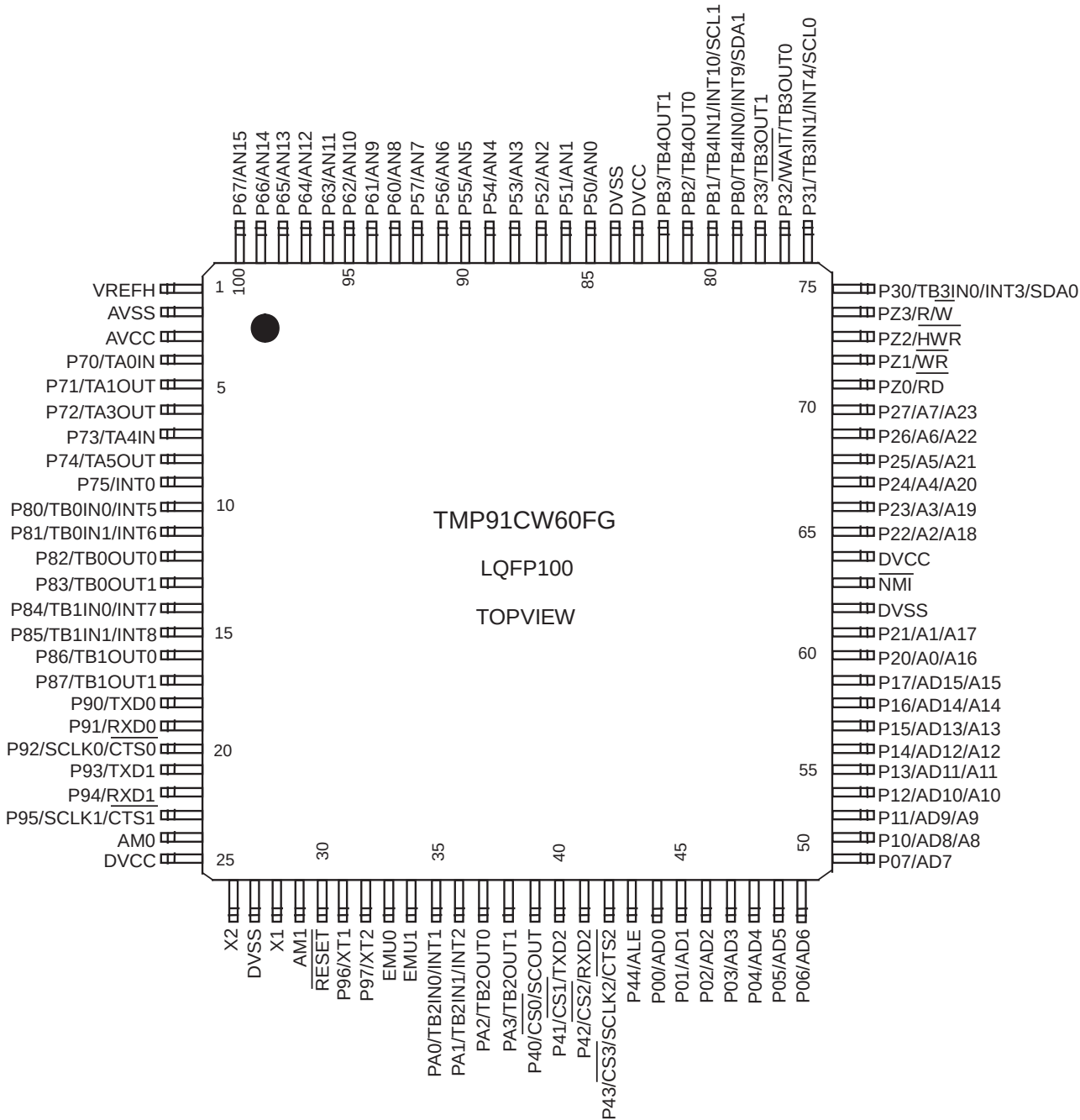
Figure 1-1 Pin Assignment(TMP91CW60FG)
