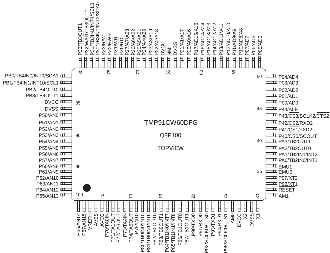
Figure 1-2 Pin Assignment(TMP91CW60DFG)
