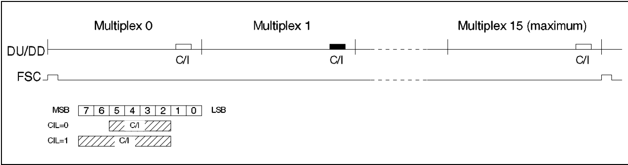
Figure 30 C/I Channels (2 Independent Channels)
