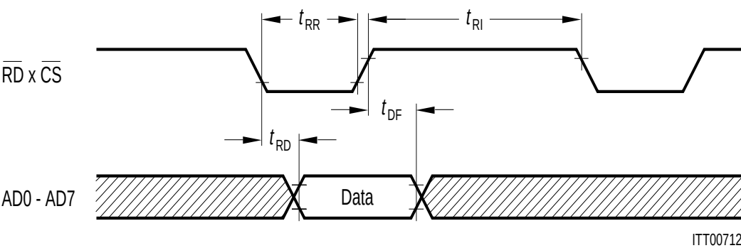
Figure 56 Microprocessor Read Timing
