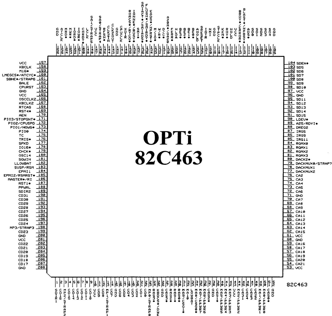
Figure 2 : OPTi 82C463 Pinout (3.3 Volts or 5 Volts only)
