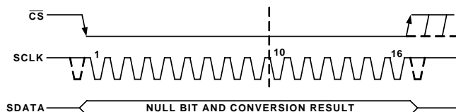
FIGURE 28. NORMAL MODE OPERATION
