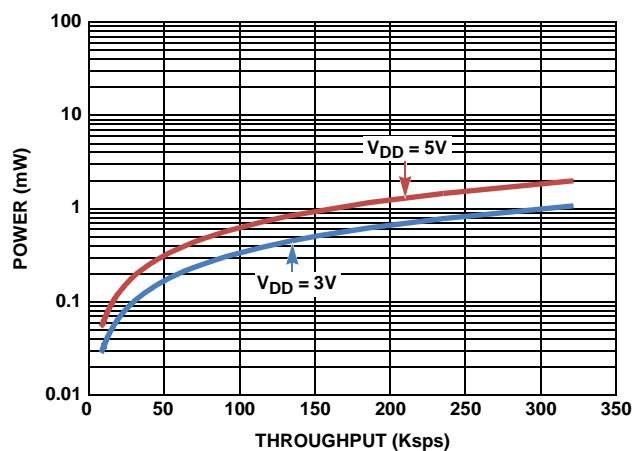
FIGURE 29. POWER CONSUMPTION vs THROUGHPUT RATE
