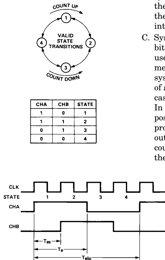
Figure 9. 4x Quadrature Decoding.
