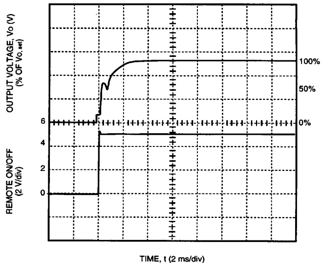
Figure 17. DC025 Triple Output-Series Typical Output Voltage Start-Up when Signal Applied to Remote On/Off
