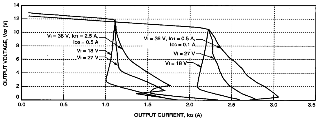
Figure 10. DC025ABK-M Typical 12 V Output Characteristics
