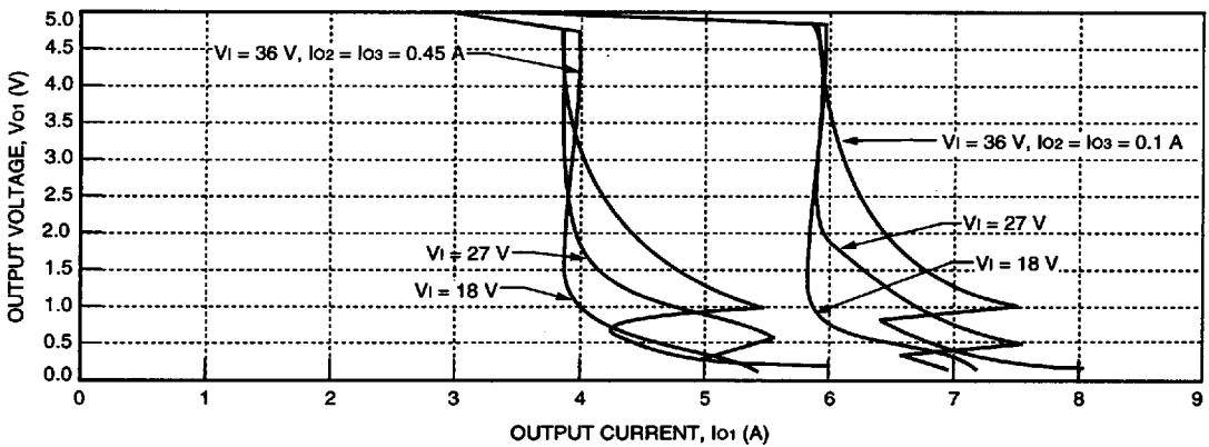
Figure 11. DC025ACL-M Typical 5 V Output Characteristics
