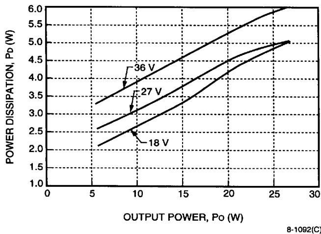
Figure 24. DC025ACL-M Fixed Losses, P_p
