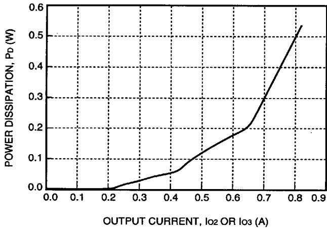
Figure 27. DC025ACL-M Losses Associated with ±15 V Output, Ps2/Ps3
