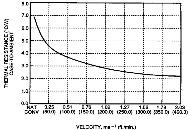
Figure 29. Case-to-Ambient Thermal Resistance vs. Air Velocity
