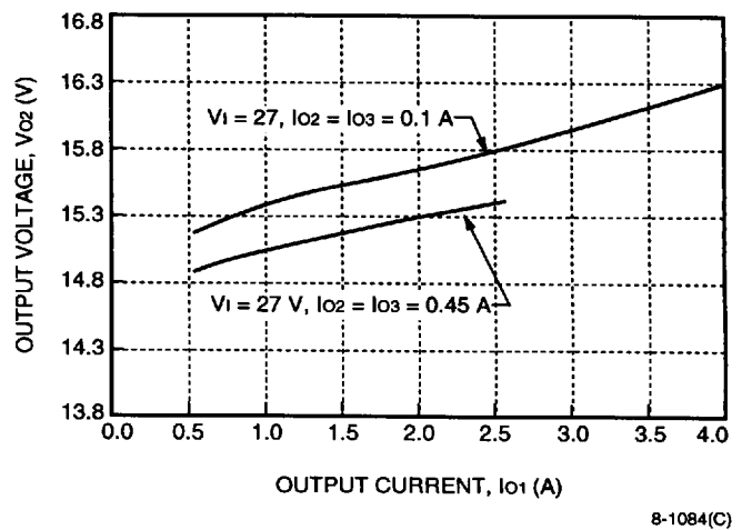
Figure 8. DC025ACL-M Typical Cross Regulation with Respect to I_{01}
