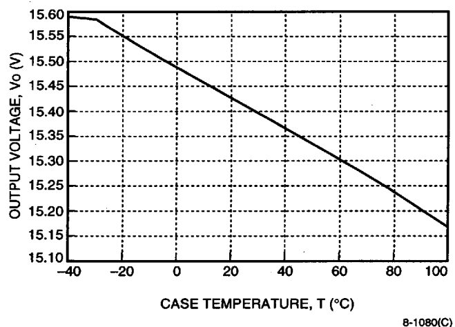
Figure 4. DC025 Triple Output-Series Typical Output Voltage Variation of 15 V Output Over Ambient Temperature Range
