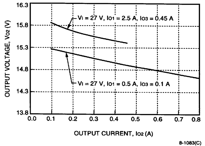
Figure 7. DC025ACL-M Typical Load Regulation
