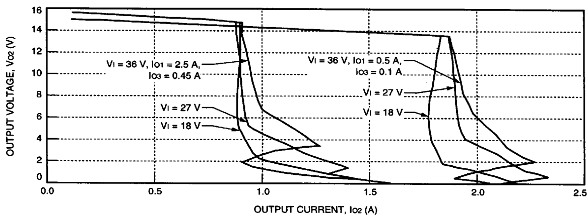
Figure 12. DC025ACL-M Typical 15 V Output Characteristics
