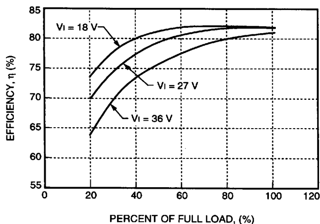
Figure 12. DC025ACL-M Typical 15 V Output Characteristics
