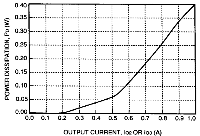
Figure 26. DC025ABK-M, Losses Associated with \pm 12 V Output, P_{s2}/P_{s3}
