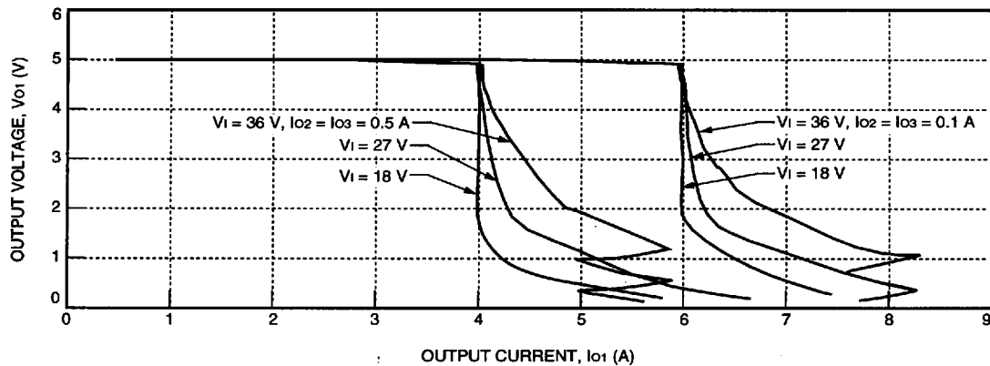
Figure 9. DC025ABK-M Typical 5 V Output Characteristics
