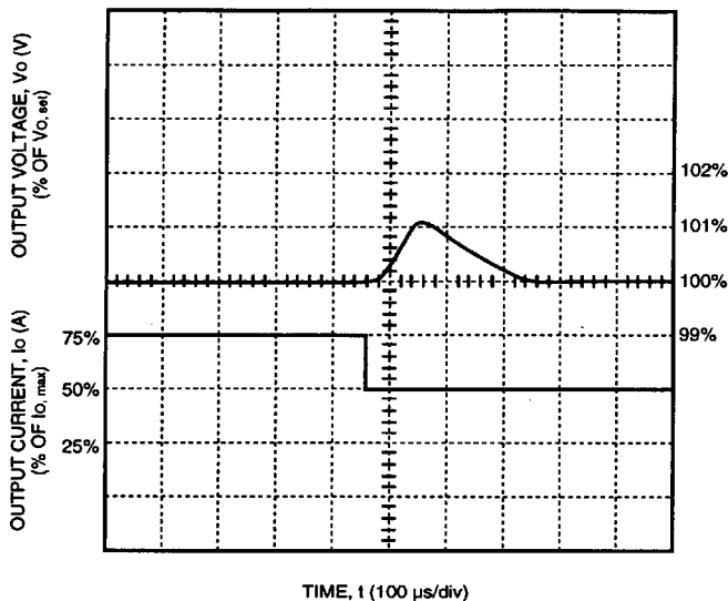
Figure 15. DC025 Triple Output-Series Typical Output Voltage for a Step Load Change from 75% to 50% of Full Load on Output 1
