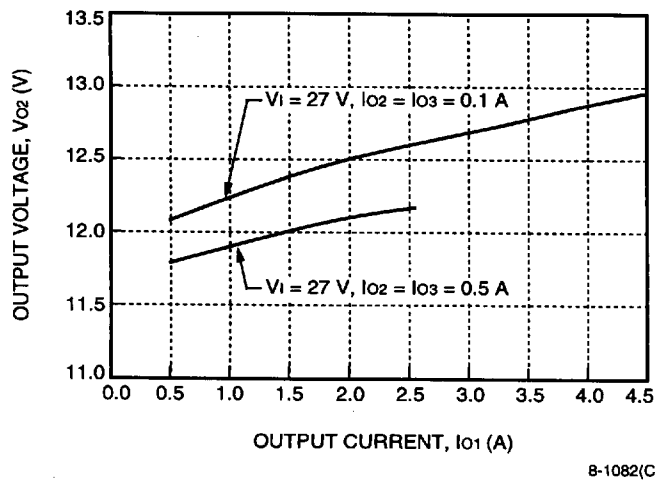
Figure 6. DC025ABK-M Typical Cross Regulation with Respect to I_{01}
