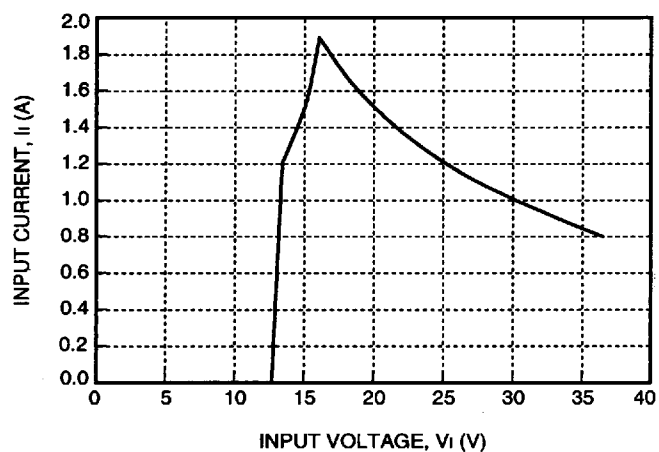
Figure 1. DC025 Triple Output-Series Typical Input Characteristics
