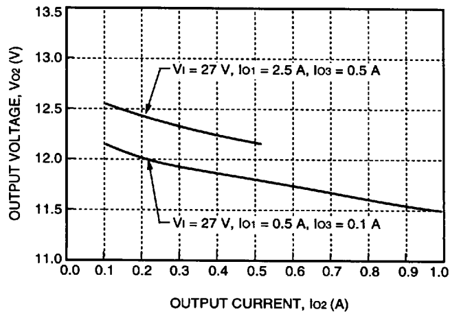
Figure 5. DC025ABK-M Typical Load Regulation
