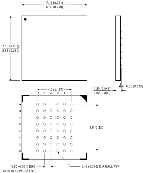
48C3 , 48-ball, Plastic Chip-size Ball Grid Array Package (CBGA) Dimensions in Millimeters and (Inches)*
