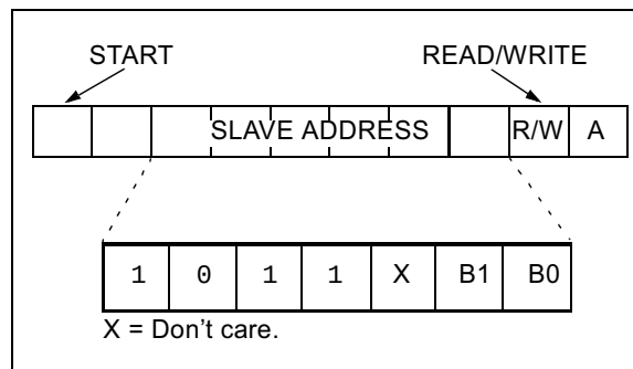
FIGURE 4-2: CONTROL BYTE ALLOCATION
