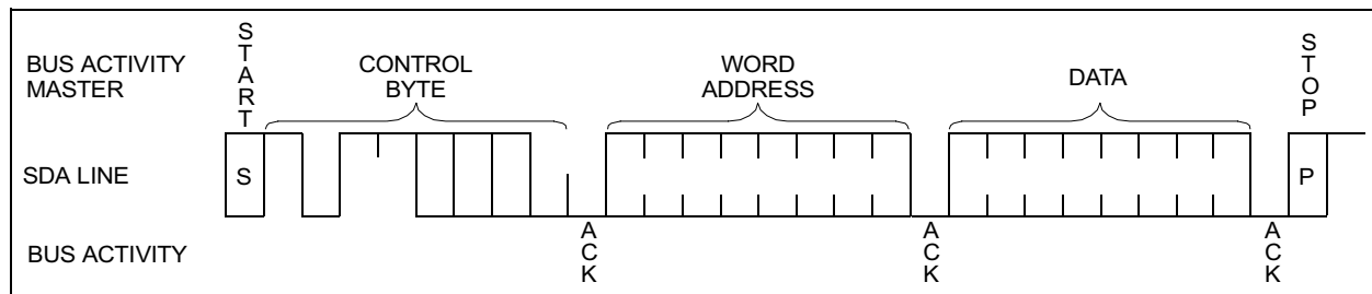
FIGURE 5-1: BYTE WRITE
