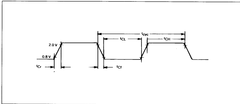
Figure 8.5 : Input Clock Waveform.
