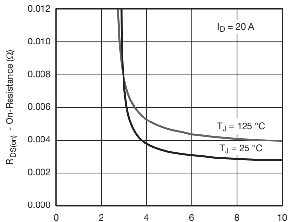
V_{GS} - Gate-to-Source Voltage (V) On-Resistance vs. Gate-to-Source
