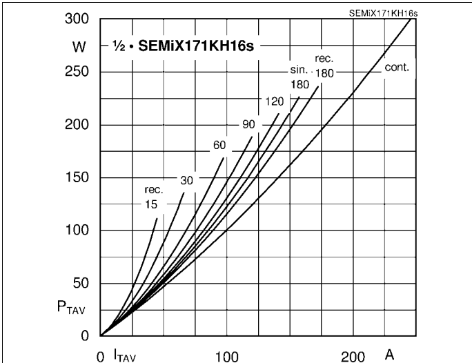
Fig. 1L: Power dissipation per thyristor/diode vs. on-state current
