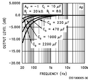
Frequency Response vs Output Capacitor Size
