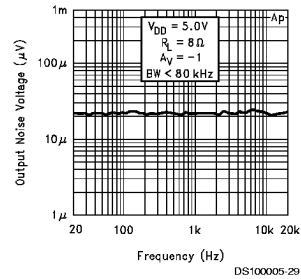
Noise Floor
