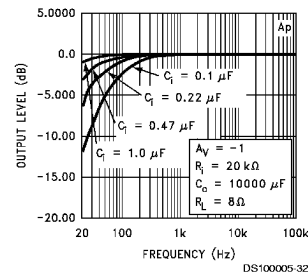
Frequency Response vs Output Capacitor Size
