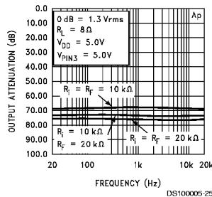
Output Attenuation in Shutdown Mode
