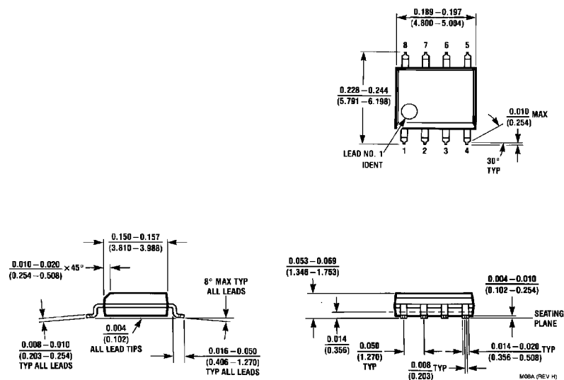
Order Number LM4881M NS Package Number M08A
