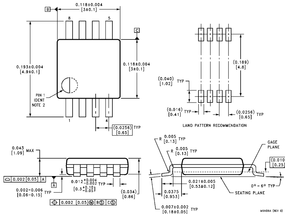
Order Number LM4881MM NS Package Number MUA08A
