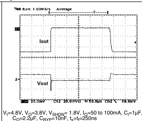
Figure 30. Load transient
