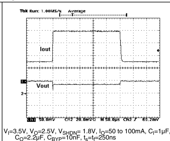
Figure 30. Load transient
