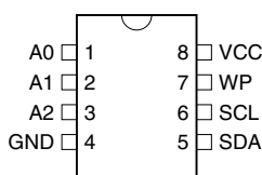
8-lead PDIP
