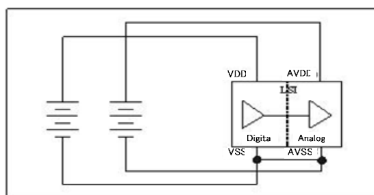
Circuit Diagram
