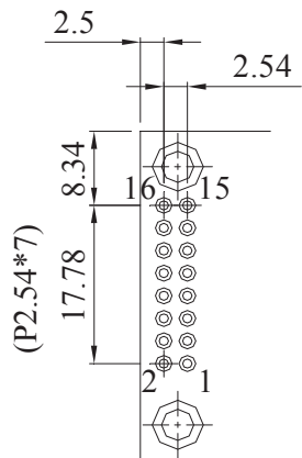
PIN DETAIL
