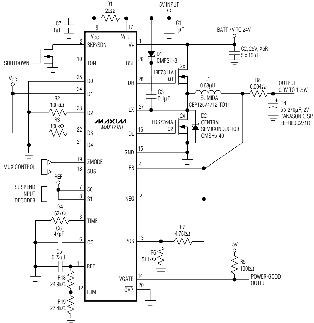
Figure 1. Standard Application Circuit
