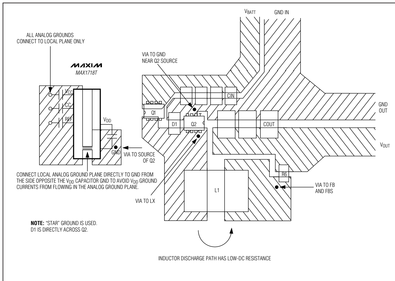
Figure 19. Power-Stage PCB Layout Example
