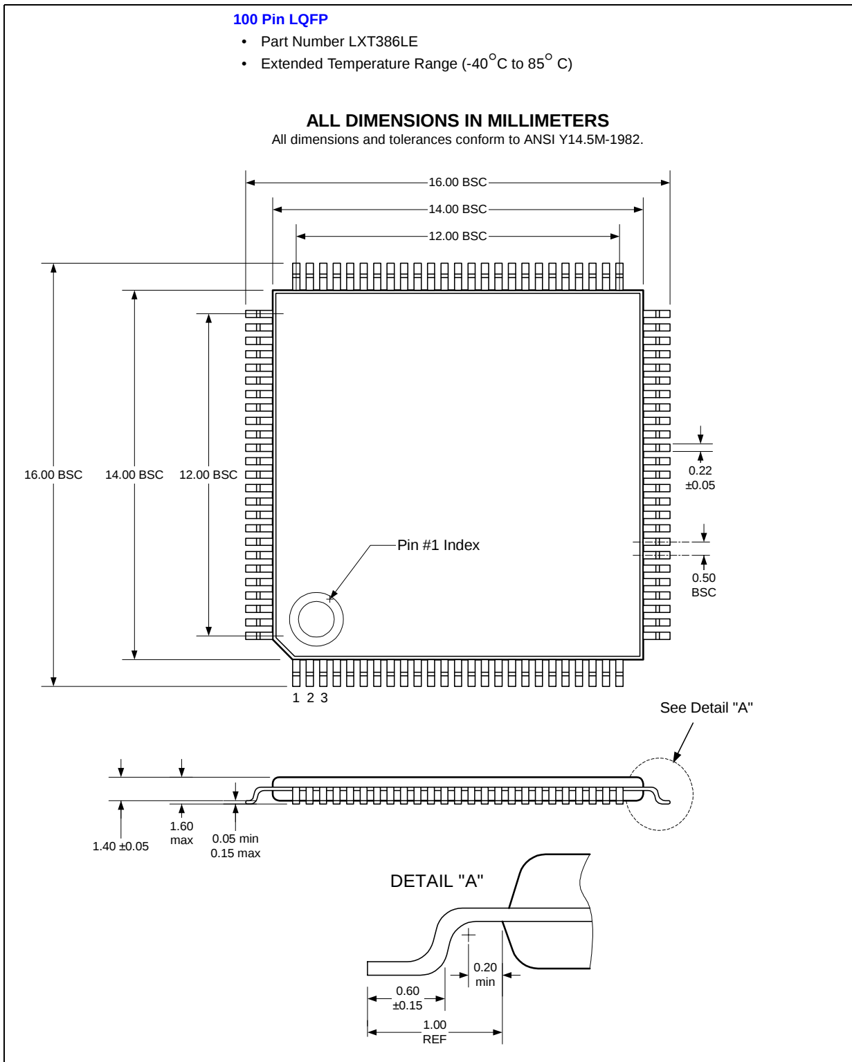
Figure 37. 100 Pin Low Quad Flat Packages (LQFP) Dimensions
