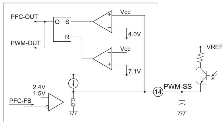
Overvoltage Latch Protection Peripheral Circuit
