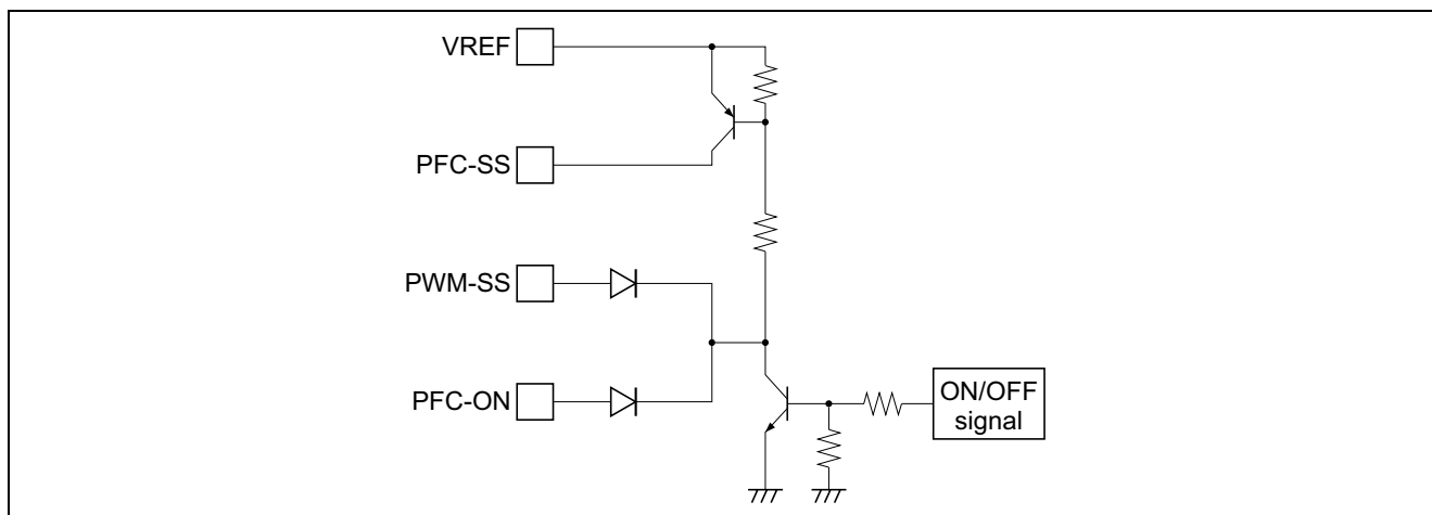
Figure 4 Example of Circuit Configuration to Turn On/Off PFC & PWM Functions
