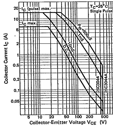
FORWARD BIAS SAFE OPERATING AREA
