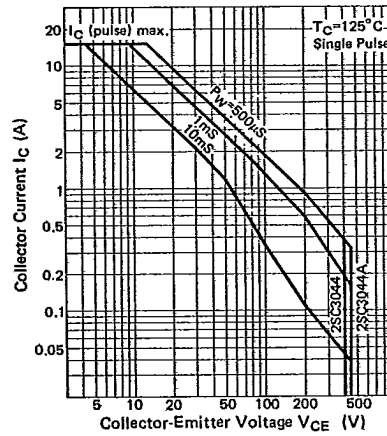
FORWARD BIAS SAFE OPERATING AREA
