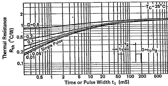
THERMAL RESPONSE
