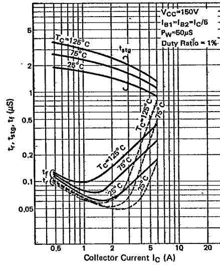
SWITCHING TIME
