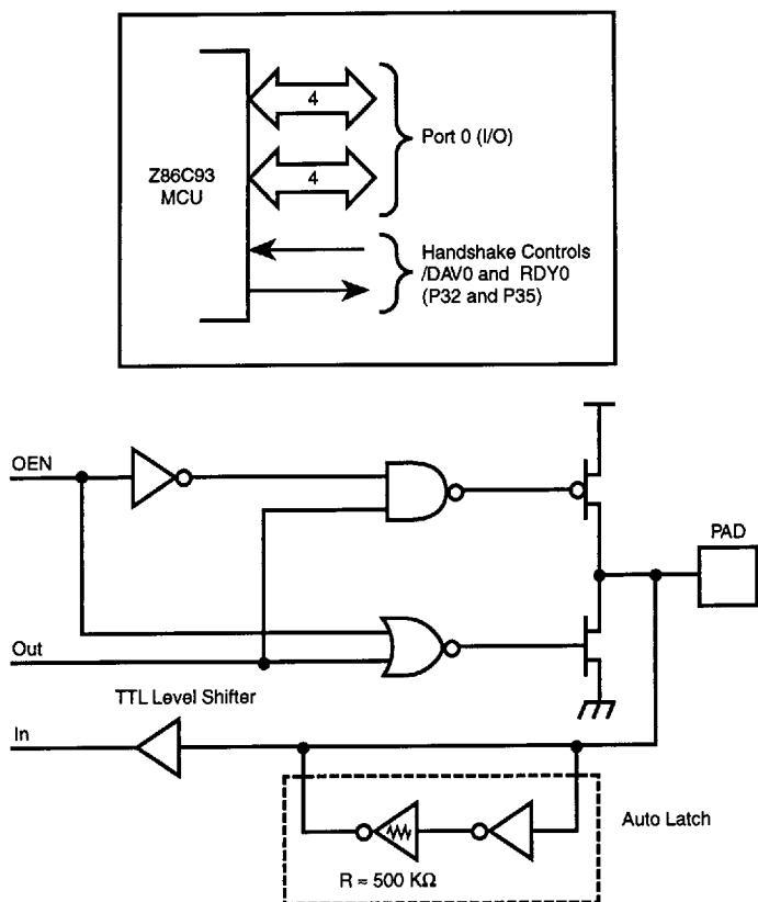
Figure 7. Port 0 Configuration
