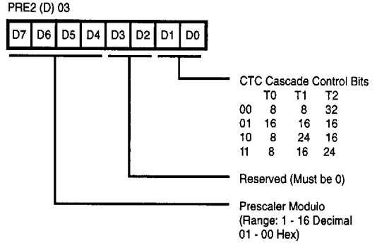
Figure 20. T2 Prescaler Register (PRE2)
