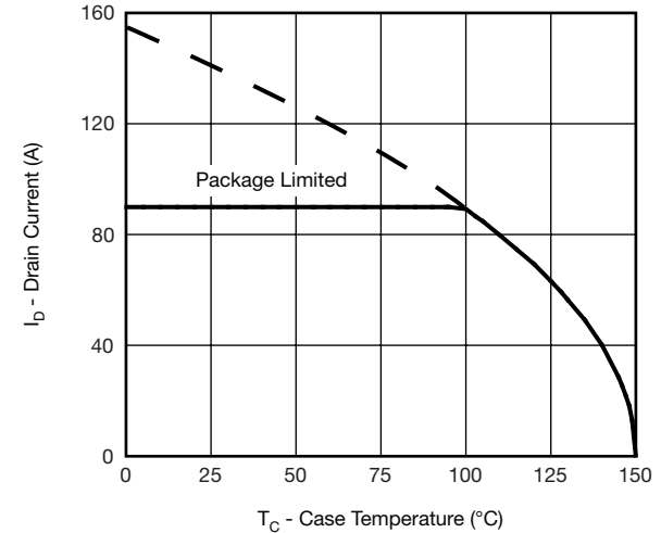
Current Derating
