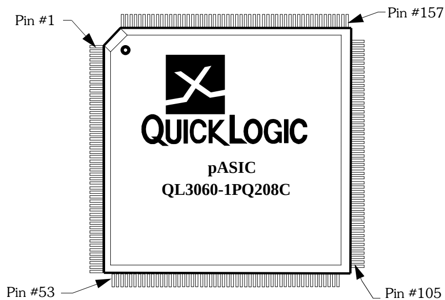
FIGURE 2. 208-Pin PQFP
