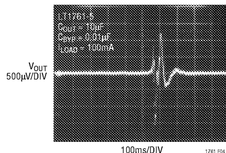
Figure 4. Noise Resulting from Tapping on a Ceramic Capacitor
