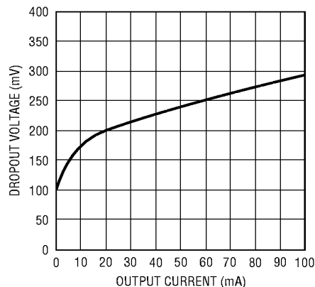
Dropout Voltage
