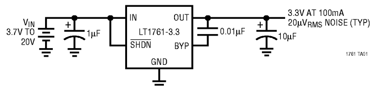
3.3V Low Noise Supply with Shutdown
