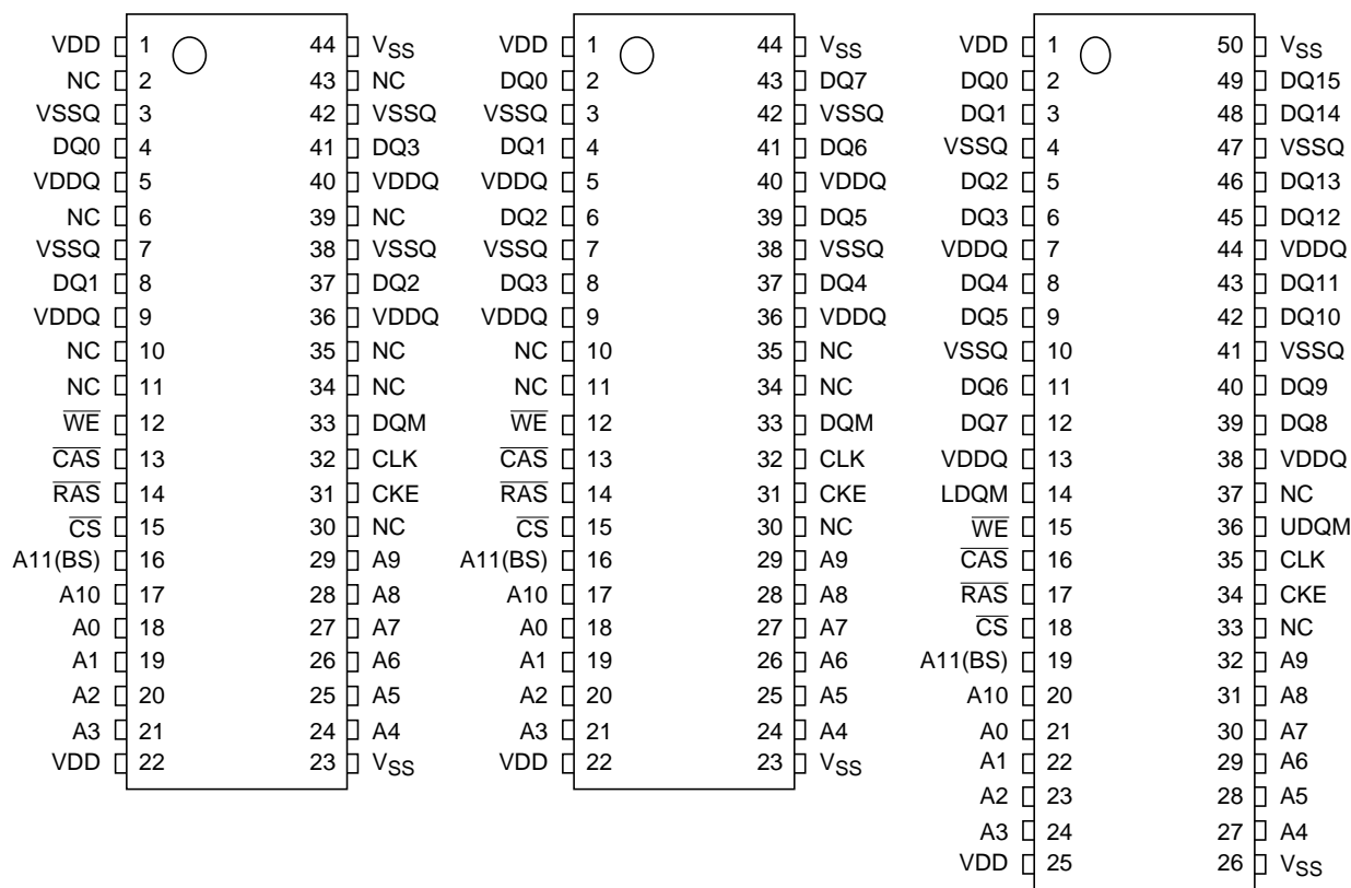
44-pin Plastic TSOP(II) 400 mil 2Mbit x 4 I/O x 2 Bank IBM0316409CT3
