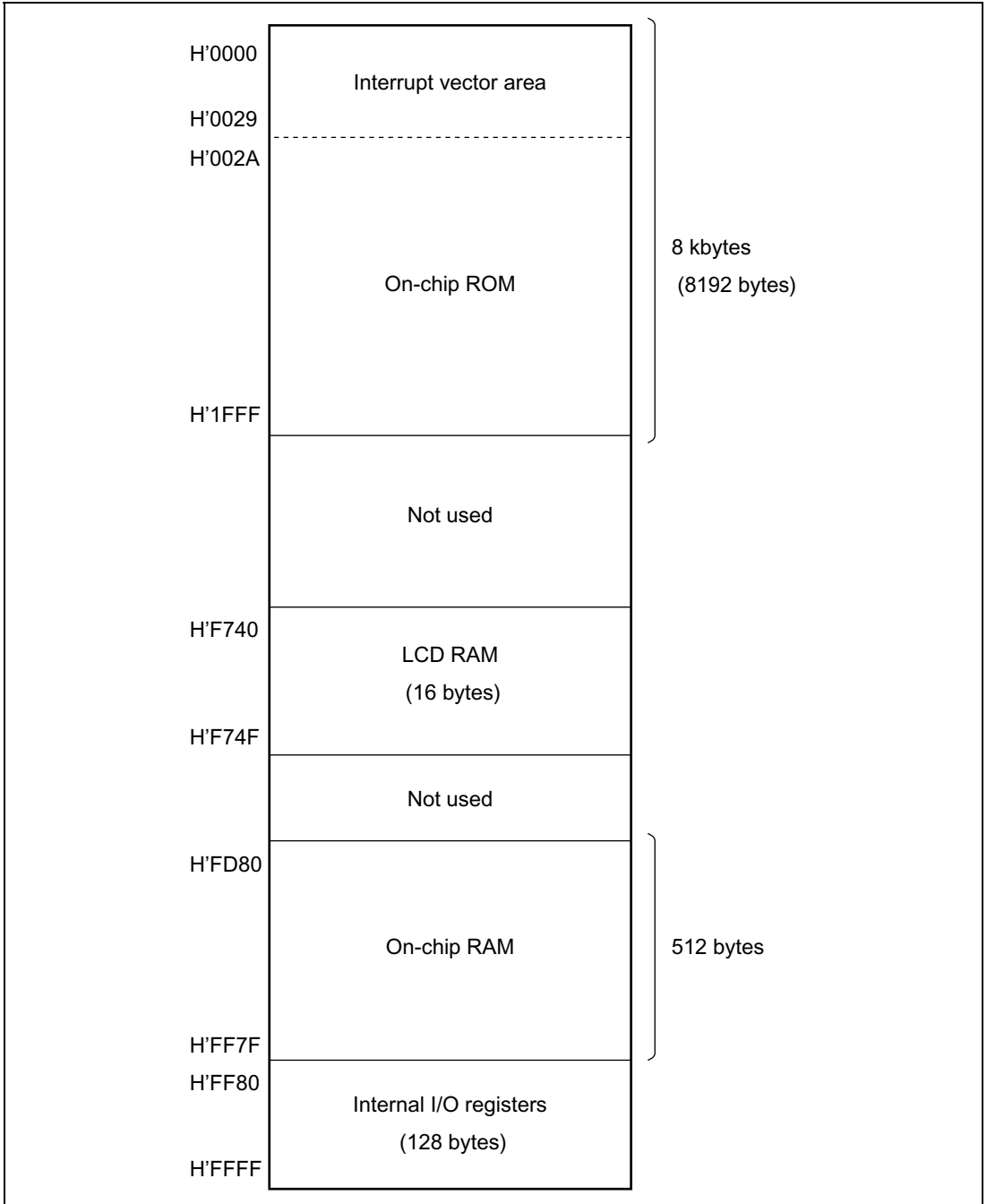
Figure 2.16(5) H8/38020 and H8/38020S Memory Map
