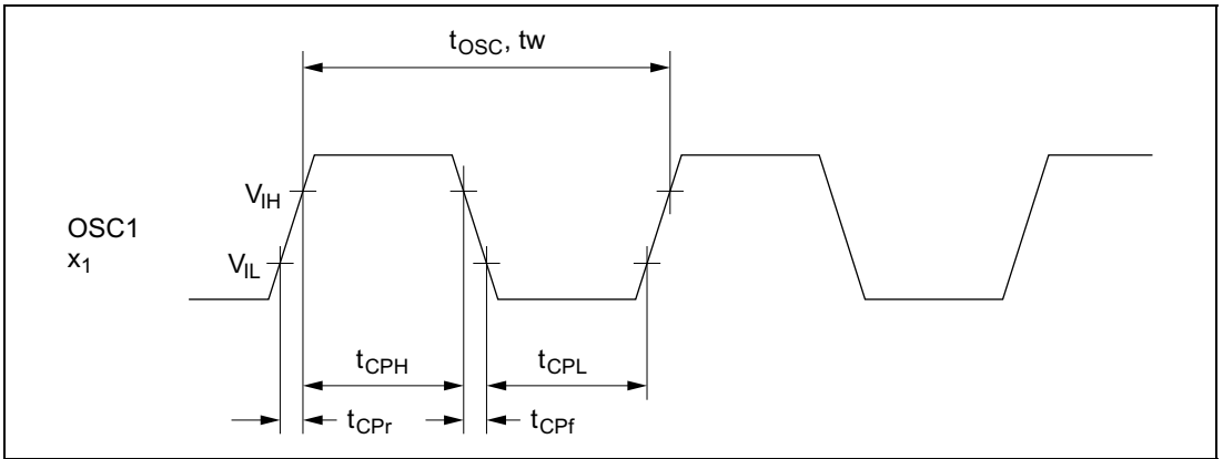
Figure 14.1 Clock Input Timing
