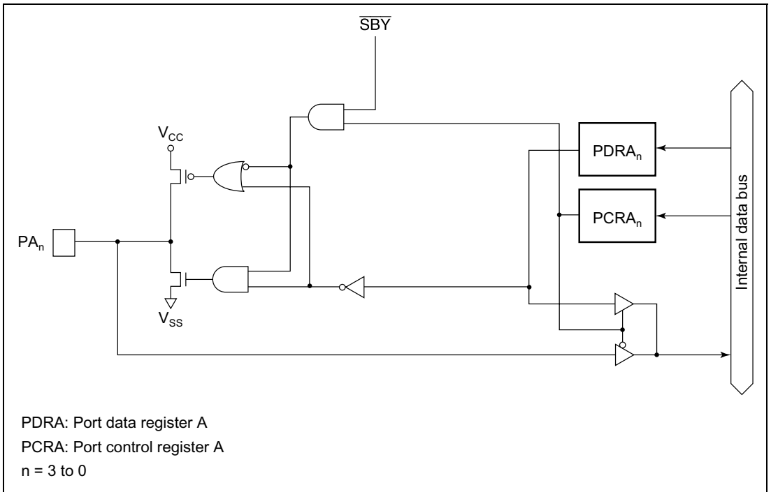
Figure C.9 Port A Block Diagram
