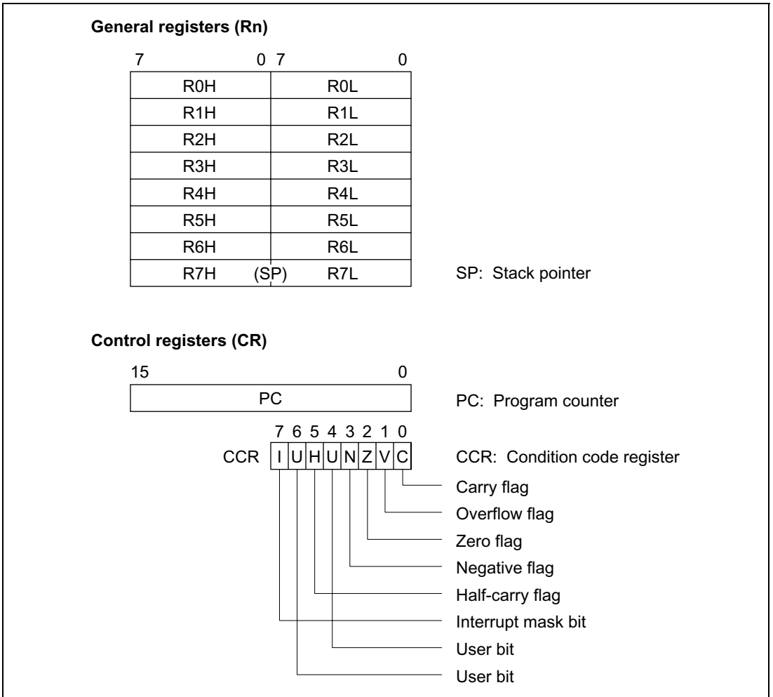
Figure 2.1 CPU Registers
