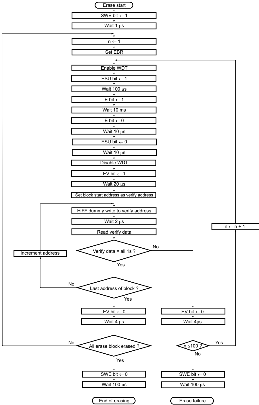
Figure 6.11 Erase/Eraser-Verify Flowchart
