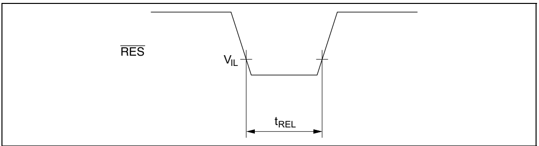
Figure 14.2 \overline{\text{RES}} Low Width
