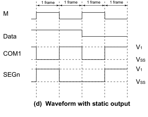
Figure 13.8 Output Waveforms for Each Duty Cycle (B Waveform)
