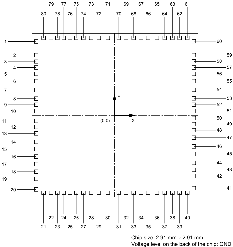
Figure 1.7 Bonding Pad Location Diagram of HCD64338024S, HCD64338023S, HCD64338022S, HCD64338021S, and HCD64338020S (Top View)
