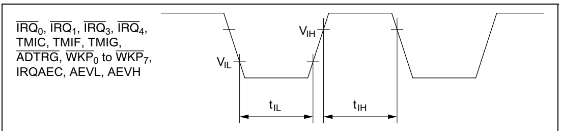
Figure 14.3 Input Timing
