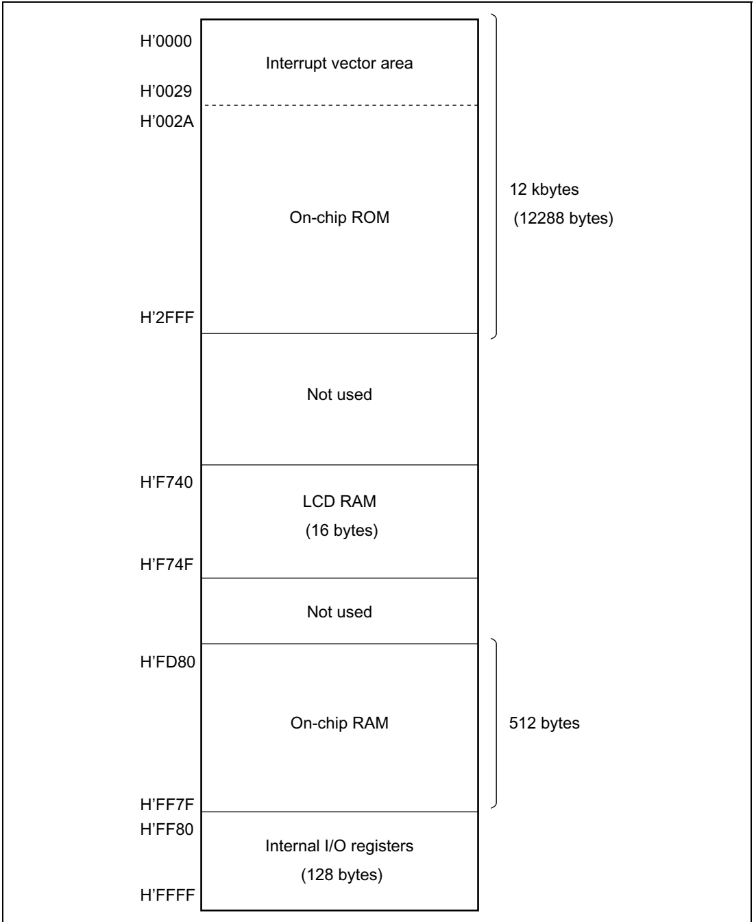
Figure 2.16(4) H8/38021 and H8/38021S Memory Map
