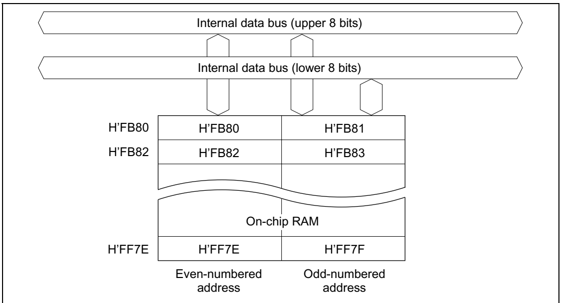
Figure 7.1 RAM Block Diagram (H8/38024)
