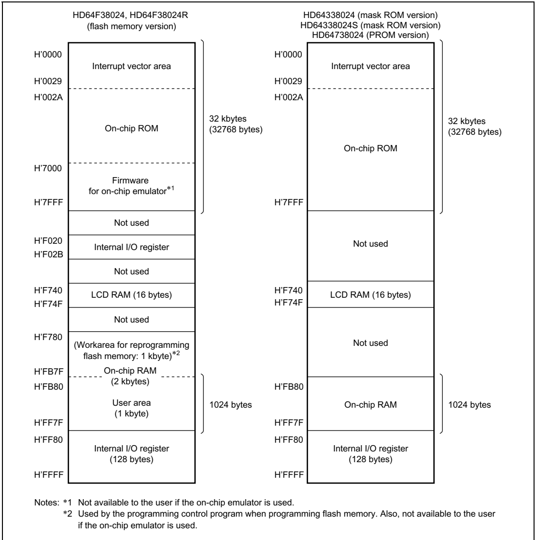
Figure 2.16(1) H8/38024 and H8/38024S Memory Map
