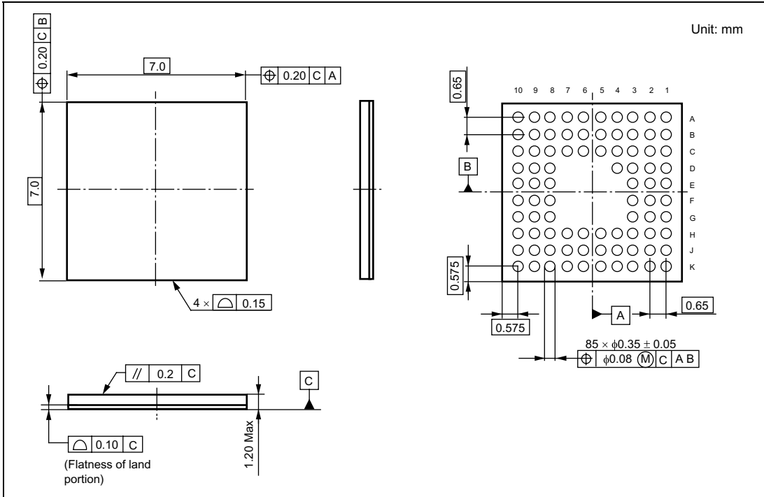
Figure F.4 TLP-85V Package Dimensions (Under development)
