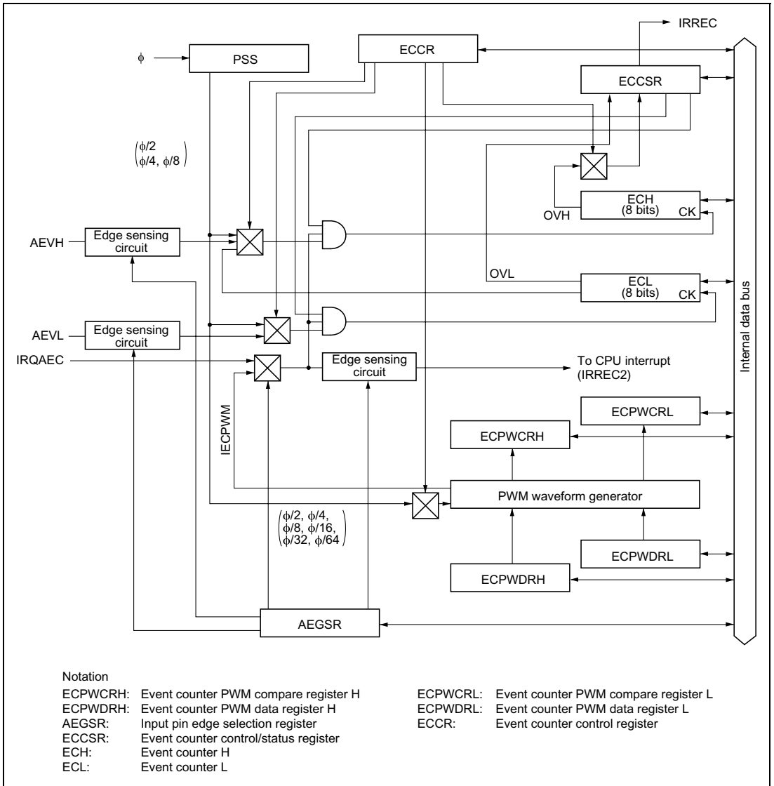
Figure 9.19 Block Diagram of Asynchronous Event Counter
