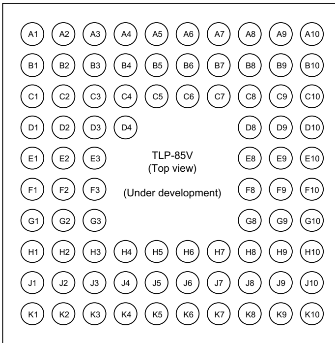
Figure 1.4 Pin Arrangement (TLP-85V) [Under Development]
