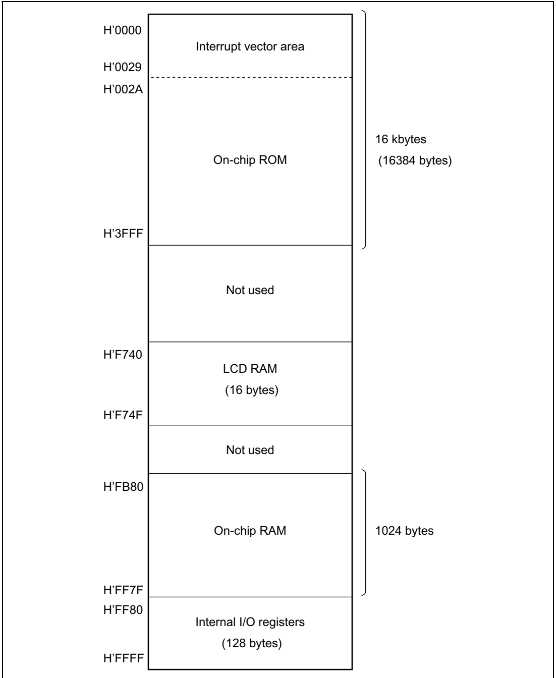
Figure 2.16(3) H8/38022 and H8/38022S Memory Map
