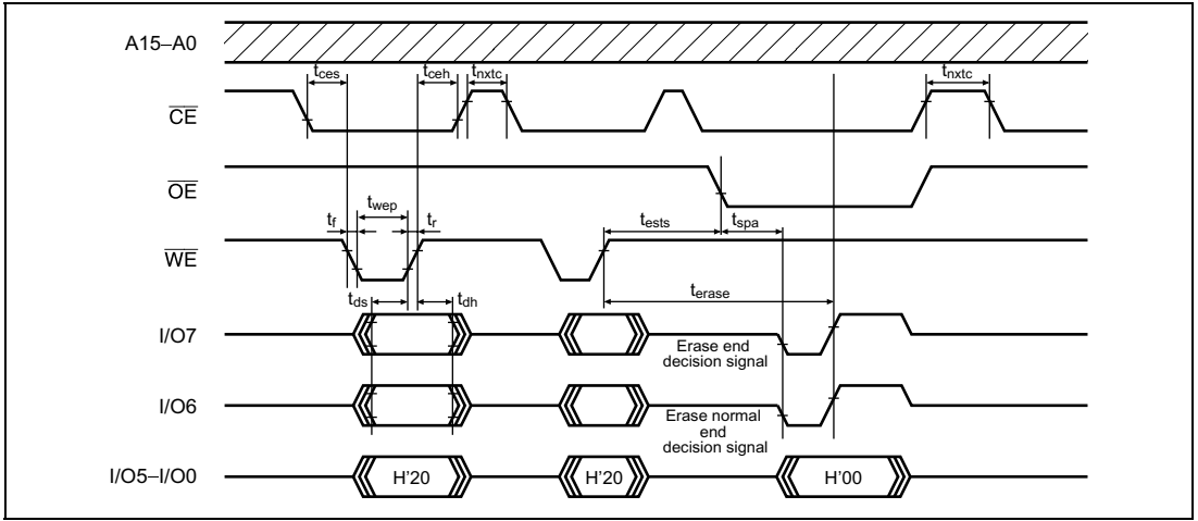
Figure 6.18 Auto-Erase Mode Timing Waveforms
