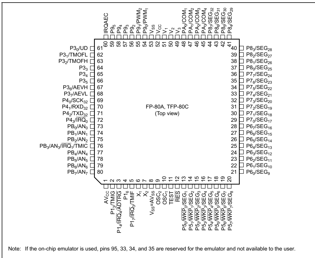
Figure 1.2 Pin Arrangement (FP-80A, TFP-80C: Top View)
