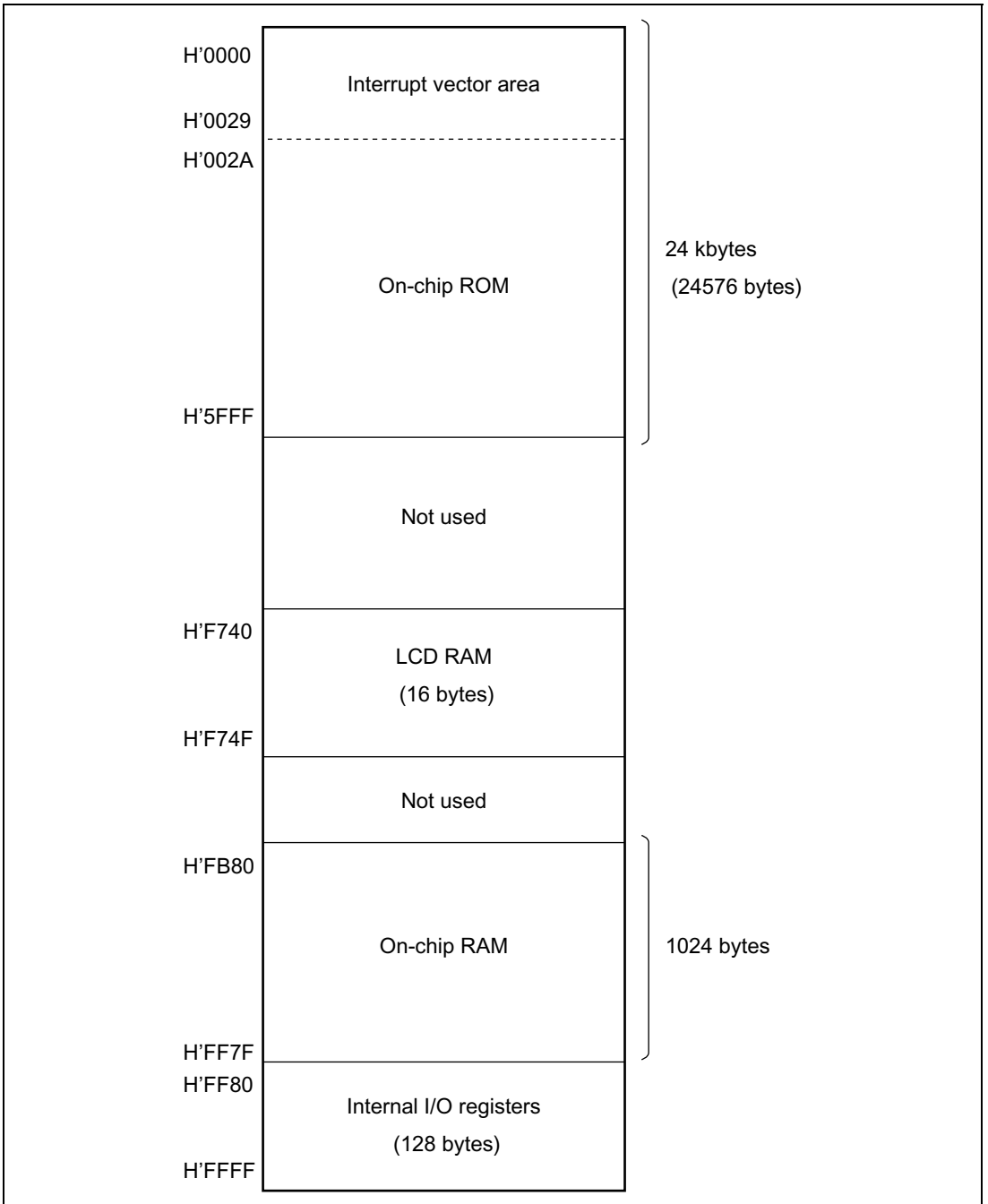
Figure 2.16(2) H8/38023 and H8/38023S Memory Map
