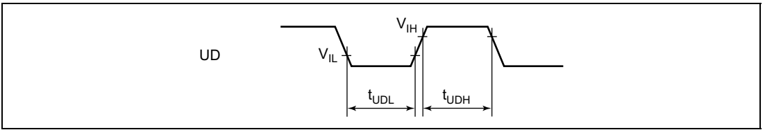
Figure 14.6 UD Pin Minimum Transition Width Timing
