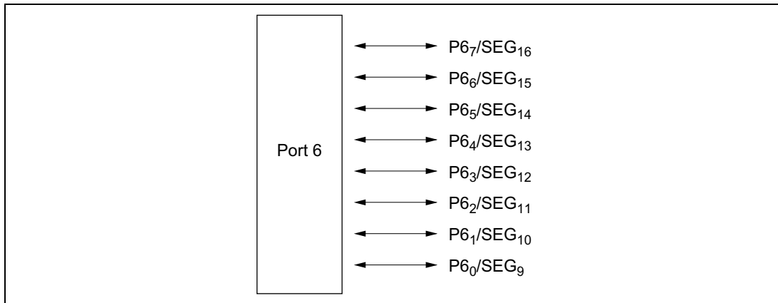
Figure 8.5 Port 6 Pin Configuration
