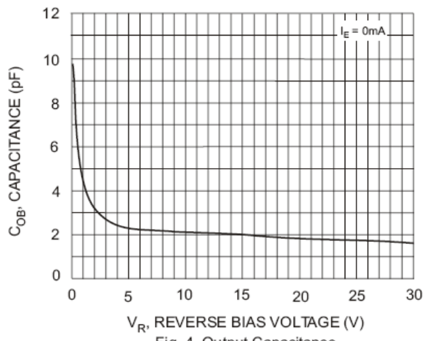
Fig. 4 Output Capacitance
