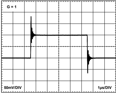
Figure 35. Small Signal Response ( G = 1 ), R_L = 10 k \Omega , C_L = 100 pF
