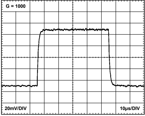
Figure 38. Small Signal Response ( G = 1000 ), R_L = 10 k \Omega , C_L = 100 pF
