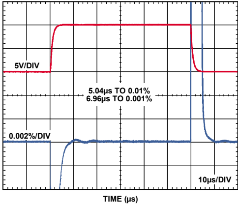
Figure 34. Large Signal Pulse Response and Settling Time ( G = 1000 ), 10 V Step, V_S = \pm 15 V
