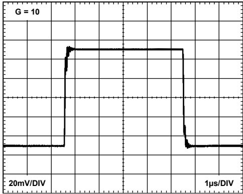
Figure 36. Small Signal Response ( G = 10 ), R_L = 10 k \Omega , C_L = 100 pF
