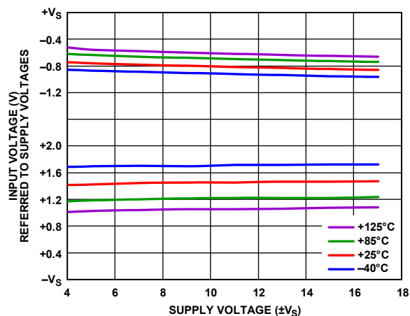
Figure 20. Output Voltage Swing vs. Supply Voltage, R_L = 10 kΩ
