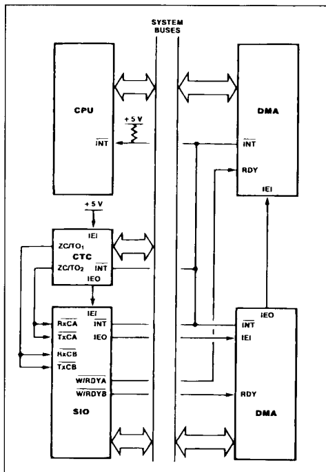
Figure 3 : Typical Z80 Environment.
