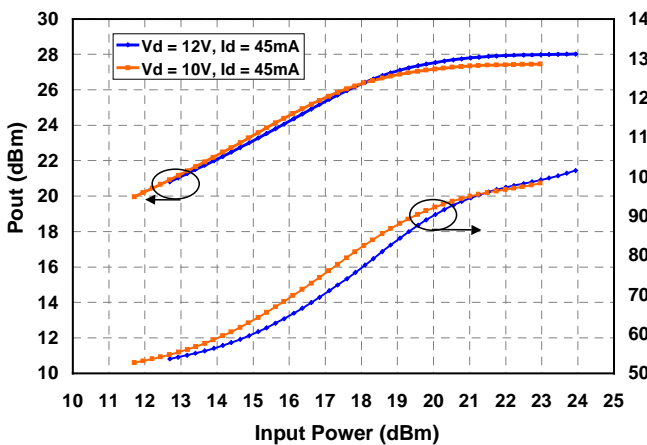
Efficiency tuned data at 18GHz
