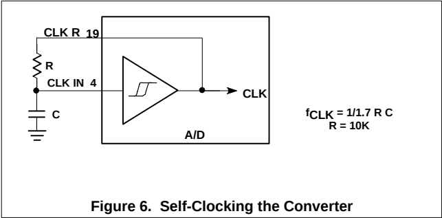
Figure 6. Self-Clocking the Converter
