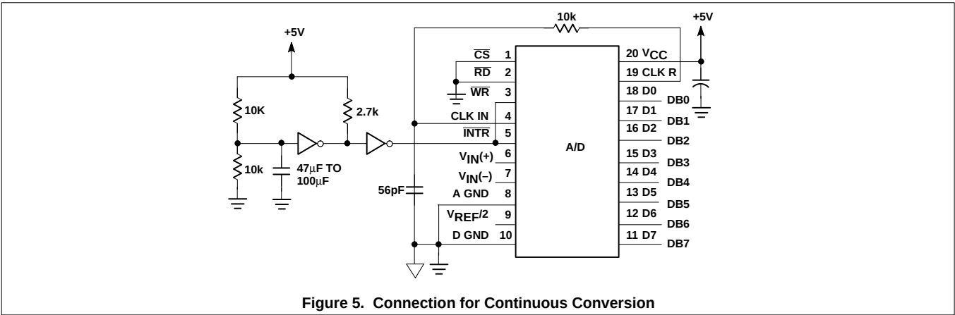
Figure 5. Connection for Continuous Conversion
