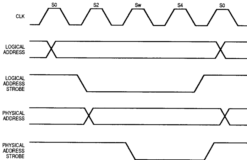
Figure 2. Address Translation Functional Timing
