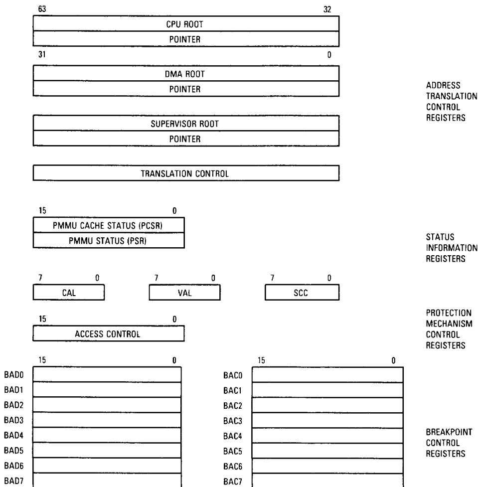
Figure 5. MC68851 Programming Model
