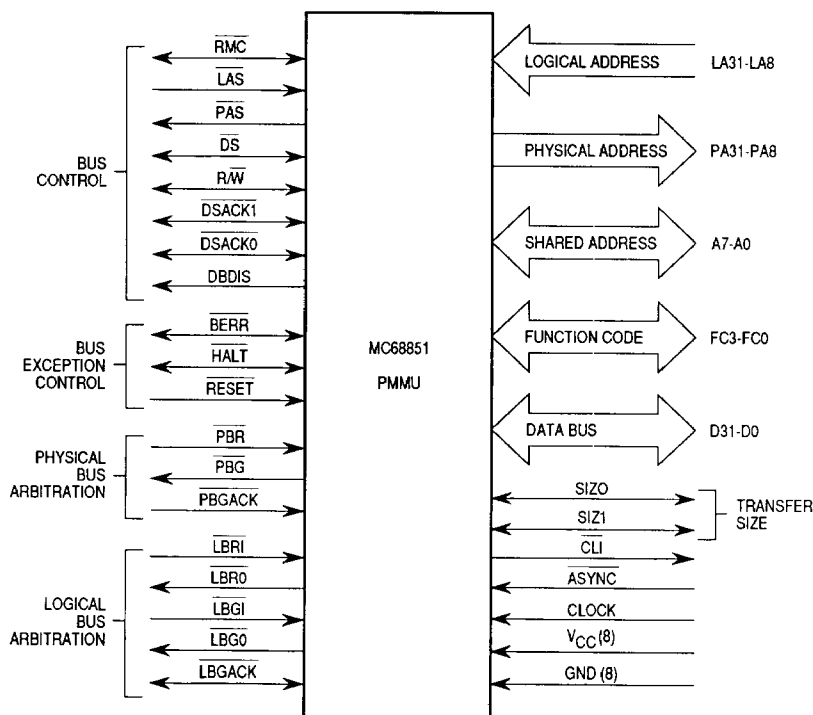
Figure 6. Functional Signal Groups
