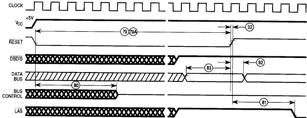
Figure 17. Reset and Mode Select Timing Diagram
