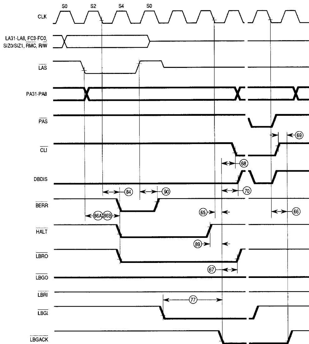
Figure 12. Logical Master Relinquish and Retry Timing Diagram
