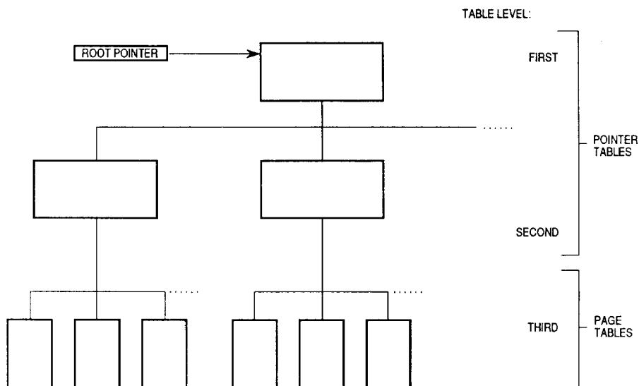
Figure 4. Translation Table Structure
