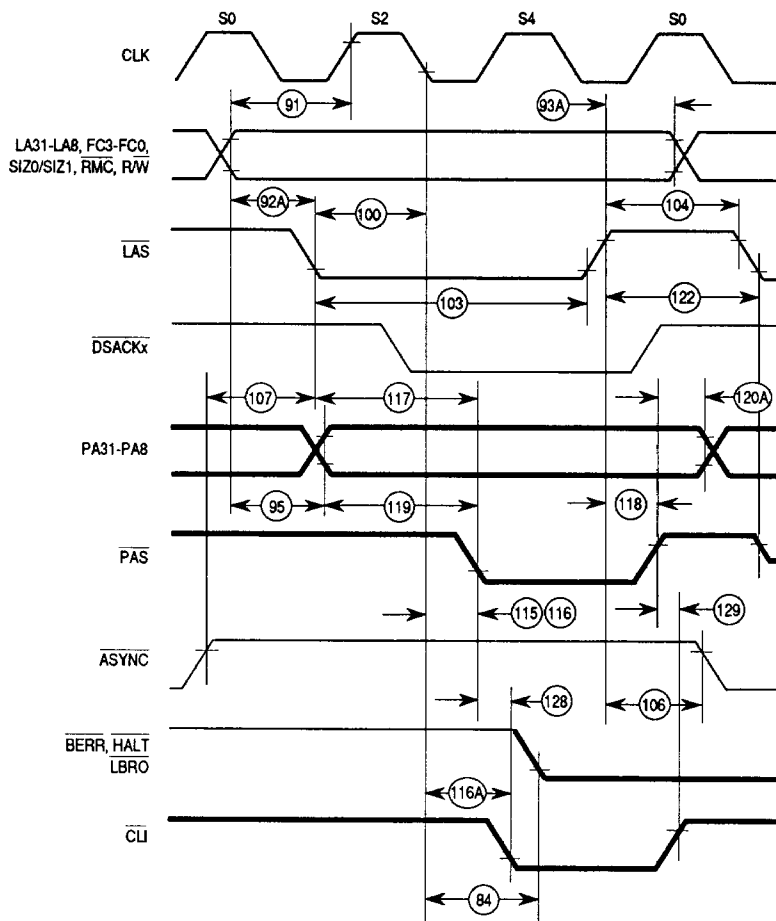
Figure 11. Synchronous Mode Translation
