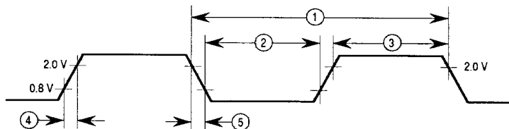
Figure 8. Clock Input Timing Diagram
