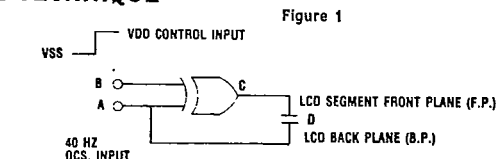
This configuration will result in a low D.C. offset A.C. drive with 2 x VDD peak value, or a RMS value equal to VDD for the LCD.
