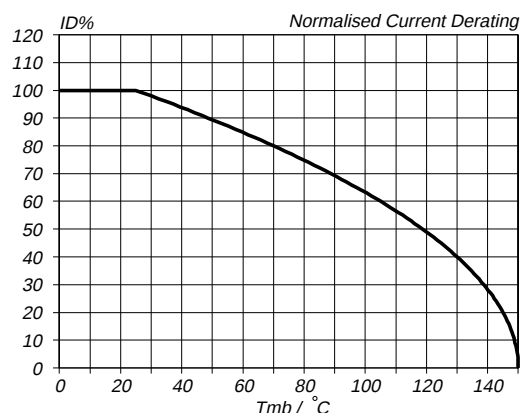
Fig.2. Normalised continuous drain current. ID\% = 100 \cdot I_D / I_{D, 25^\circ\text{C}} = f(T_{sp}) ; conditions: V_{GS} \geq 5\text{ V}
