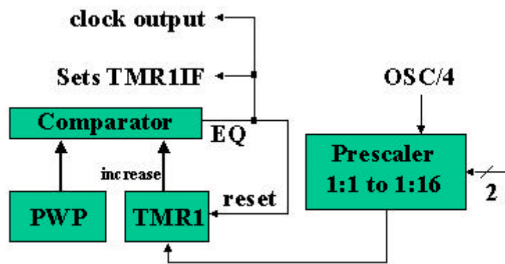
Fig. 15 TIMER1 Block Diagram
