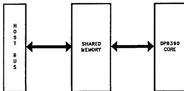
FIGURE 2. Shared Memory
