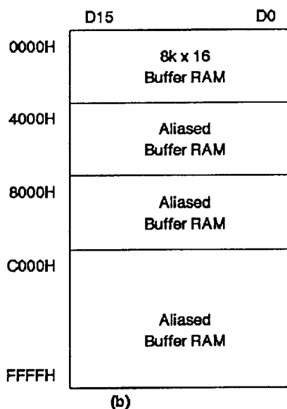
FIGURE 3. Shared Memory Mode a) Register Mapping and b) NIC Core Memory Map
