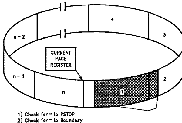
FIGURE 31. Linking Receive Buffer Pages
