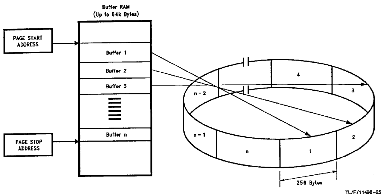
FIGURE 28. AT/LANTIC Controller Receiver Buffer Ring
