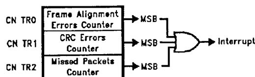
FIGURE 36. Tally Counters
