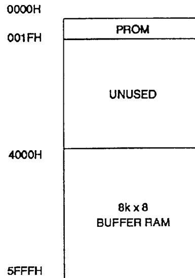
FIGURE 7. I/O Mode DP8390 Core Memory Map
