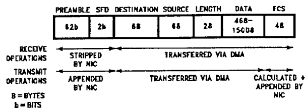
FIGURE 26. Ethernet Packet
