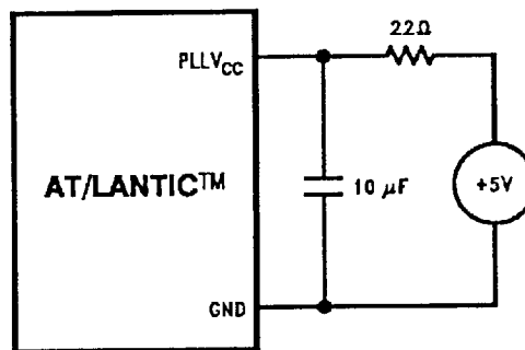
FIGURE 22. Filtering Power Supply Noise
