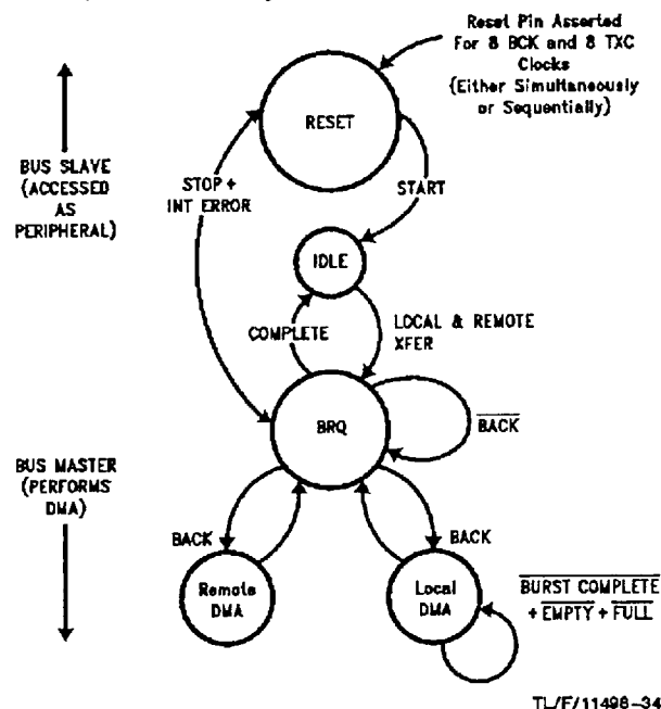
FIGURE 37. DP8390 Core Bus States
