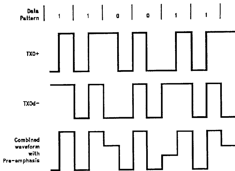
FIGURE 15. Typical Summed Transmit Waveform
