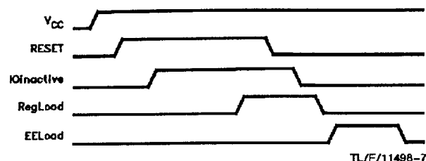
FIGURE 9. RESET Operation
