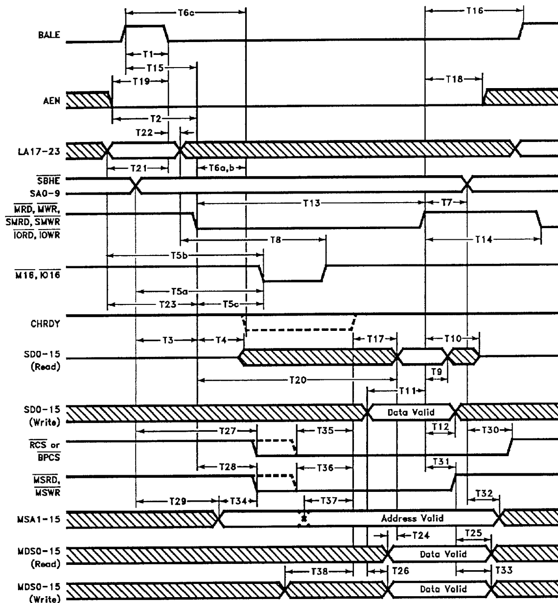
ISA Slave Accesses
