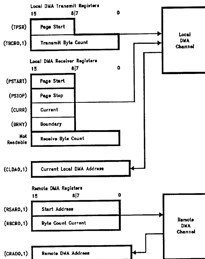
FIGURE 24. DMA Register
