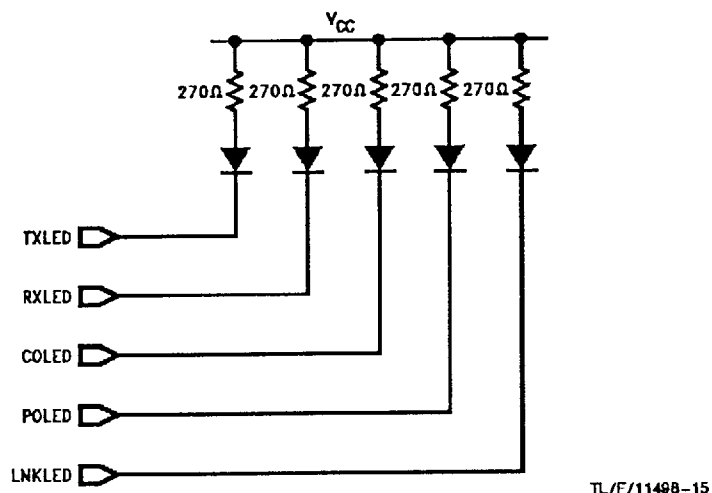
FIGURE 17. Typical AT/LANIC™ Controller LED Connection
