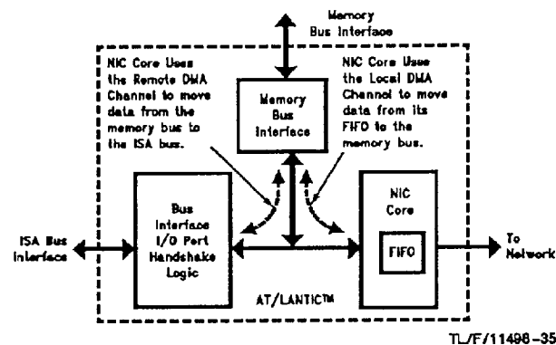
FIGURE 38. I/O Operation: All Data Transfers and Arbitration is Controlled by the NIC Core
