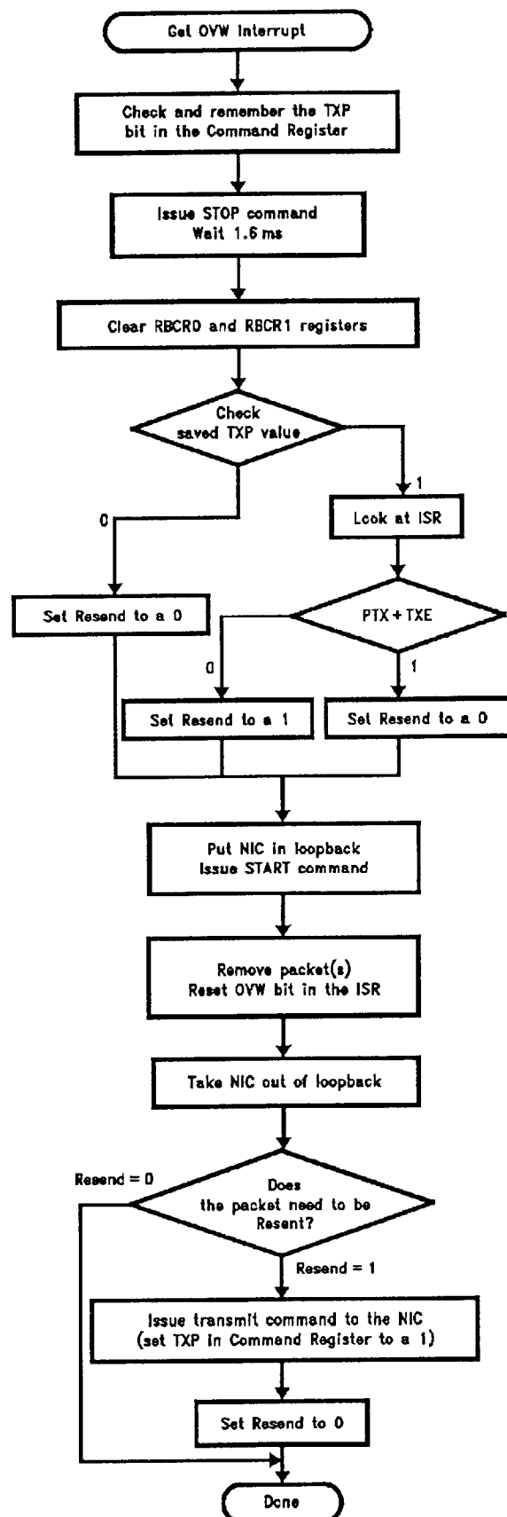
FIGURE 32. Overflow Routine
