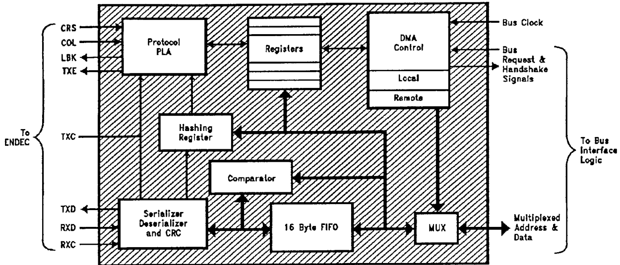
FIGURE 12. DP8390 Controller Core Simplified Block Diagram
