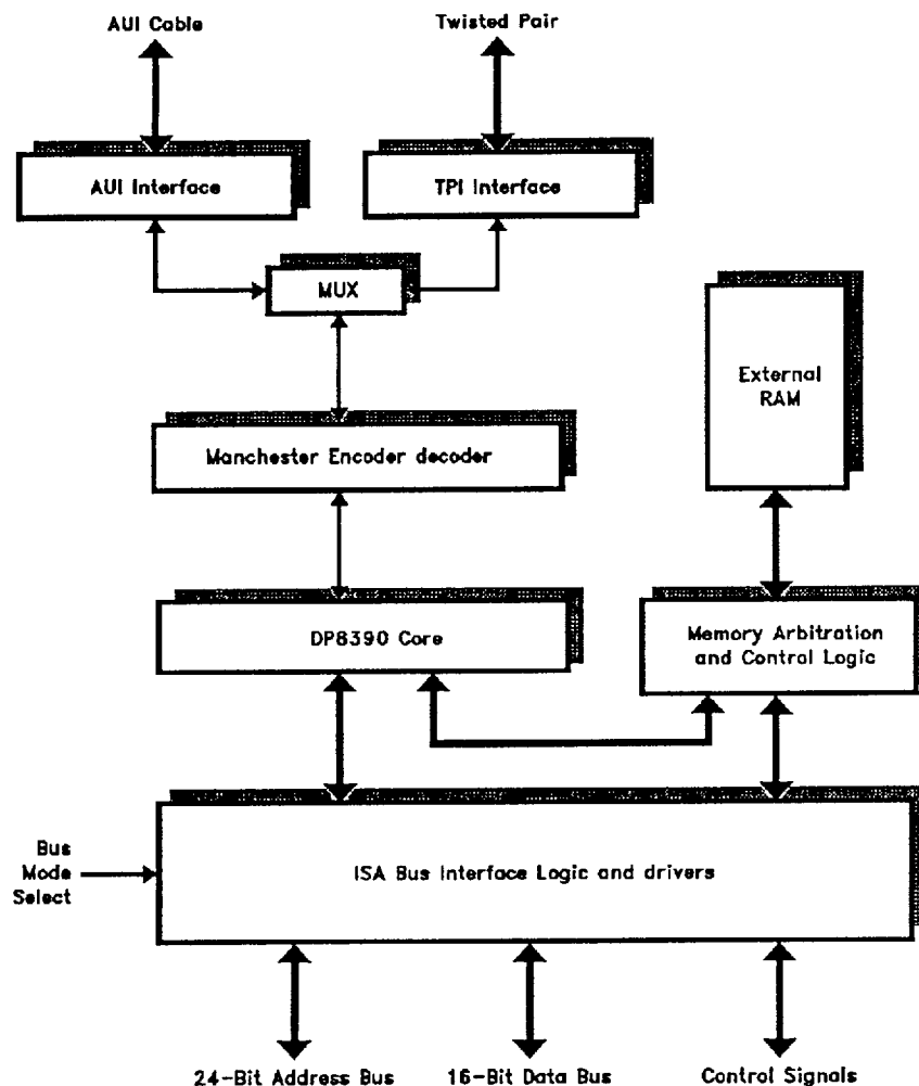
FIGURE 1. Block Diagram of AT/LANTIC Controller
