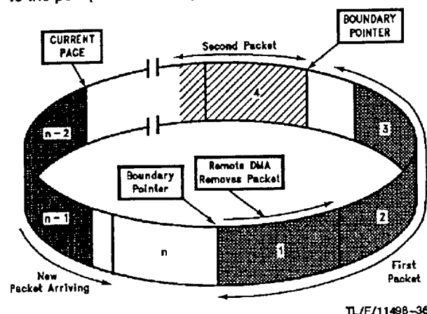
FIGURE 39. 1st Received Packet Removed by Remote DMA
