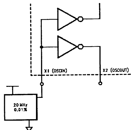
FIGURE 20. AT/LANTIC Controller Connection for Oscillator Module
