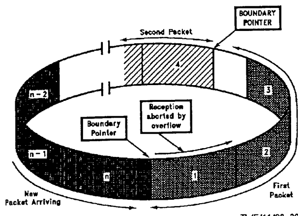
FIGURE 33. Received Packet Aborted If It Hits Boundary
