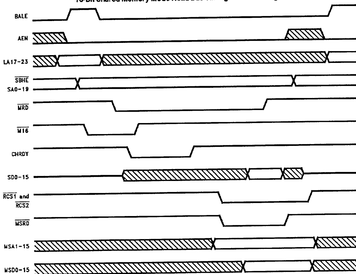
16-Bit Shared Memory Mode Read Bus Timing with DWID High
