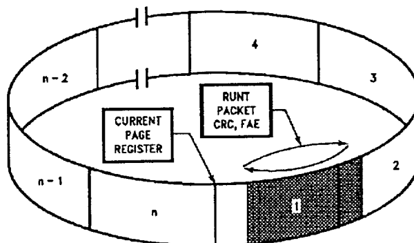
FIGURE 35. Termination of Receive Packet—Packet Reject
