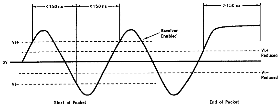
FIGURE 14. Twisted Pair Squelch Waveform
