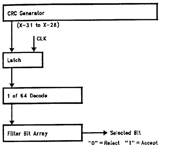
FIGURE 25. Multicast Addressing
