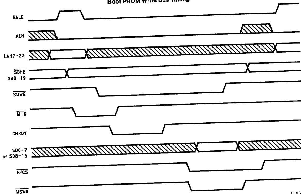
Boot PROM Write Bus Timing
