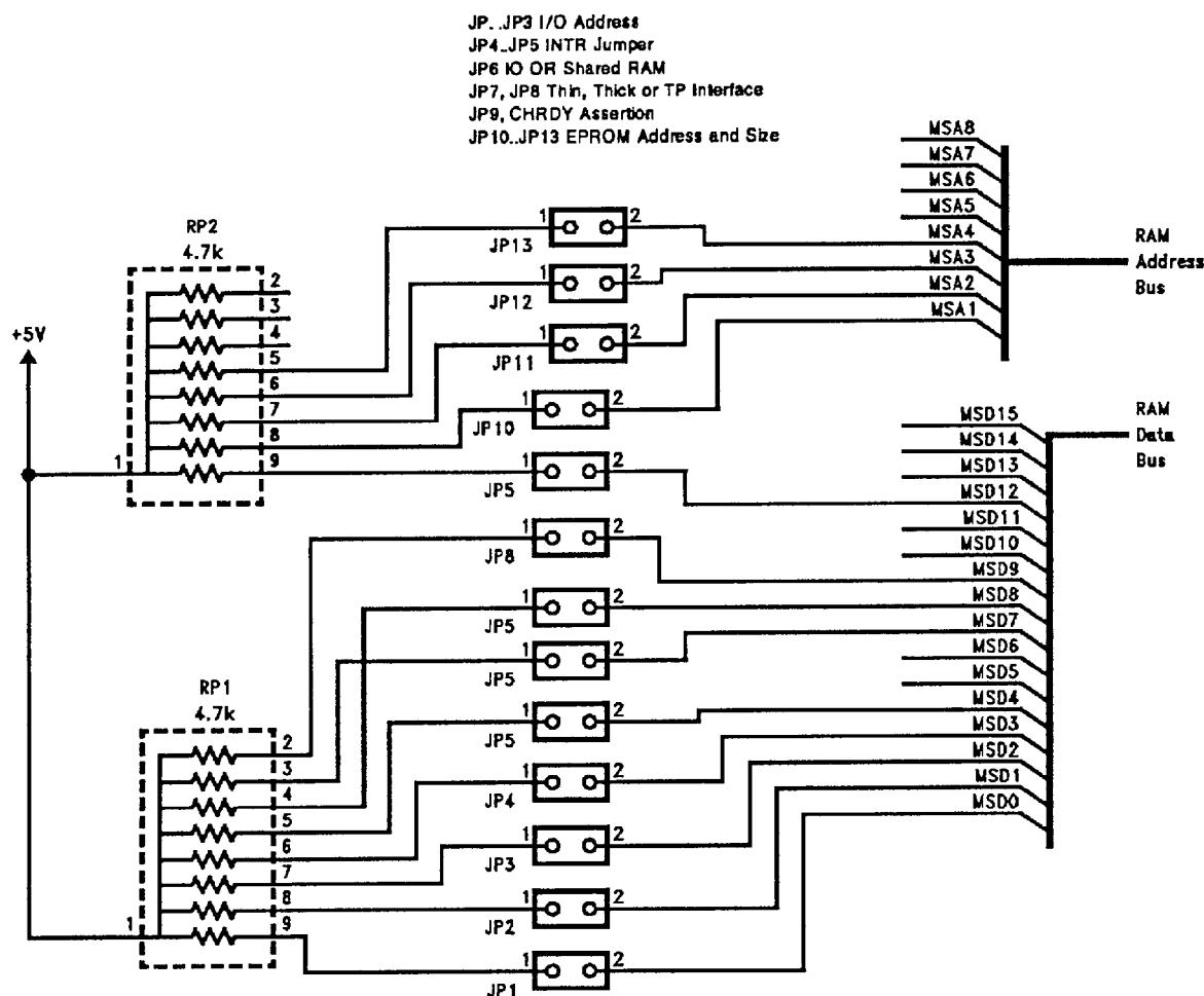
FIGURE 11. Example of Jumper Configuration
