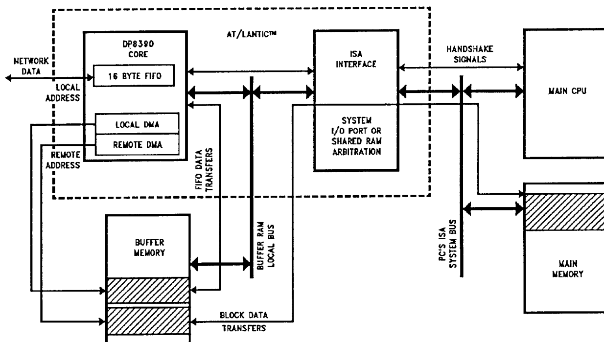
FIGURE 27. AT/LANTIC Controller Bus Architecture
