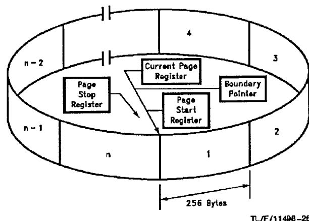
FIGURE 29. Buffer Ring at Initialization
