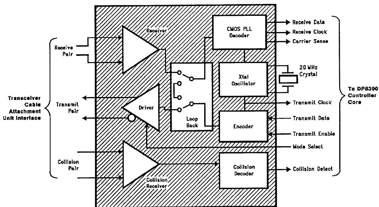
FIGURE 18. Encoder/Decode Block Diagram
