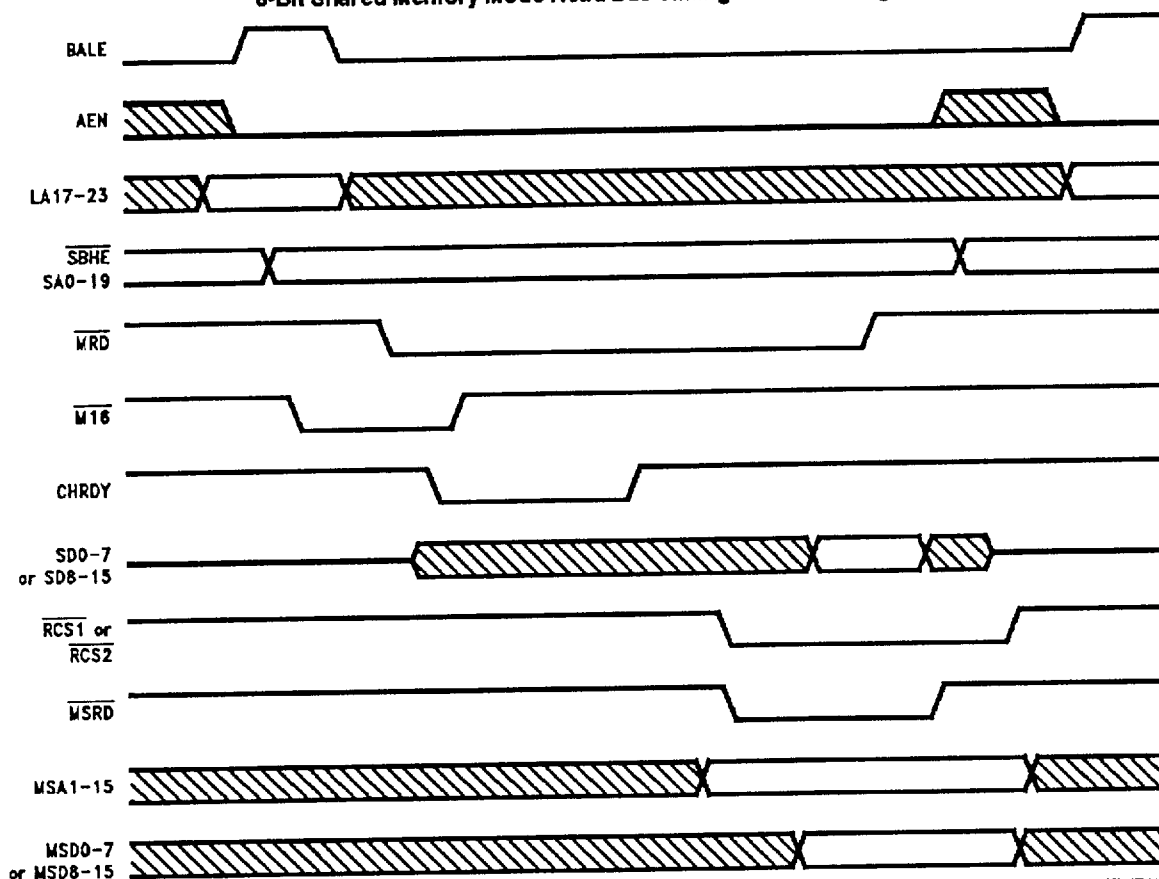
8-Bit Shared Memory Mode Read Bus Timing with DWID High
