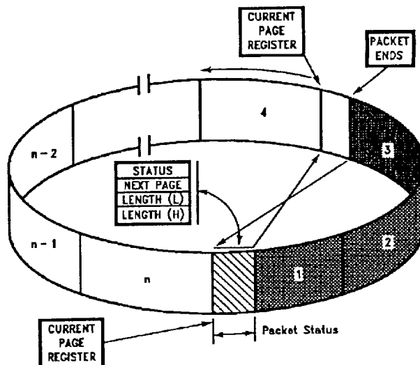
FIGURE 34. Termination of Received Packet—Packet Accepted
