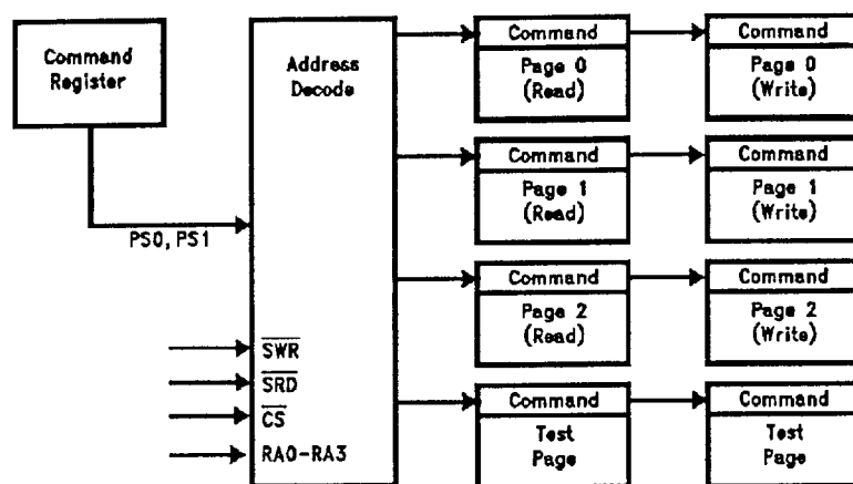
FIGURE 23. NIC Core Register Mapping
