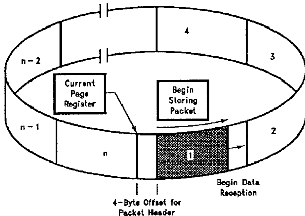
FIGURE 30. Received Packet Enters the Buffer Pages
