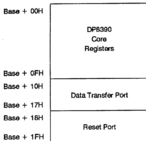
FIGURE 5. I/O Port Mode Register I/O Map
