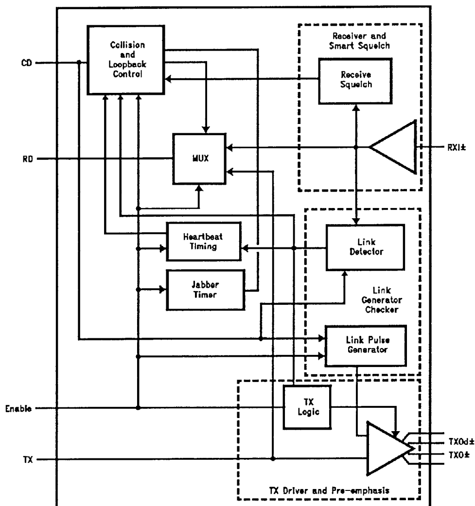
FIGURE 13. Twisted Pair Interface Module Block Diagram
