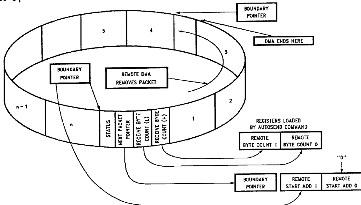
FIGURE 40. Remote DMA AutoInitialization from Buffer Ring
