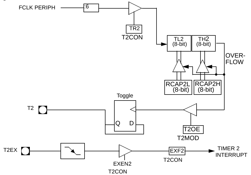
Figure 15. Clock-out Mode \overline{C/T2} = 0
