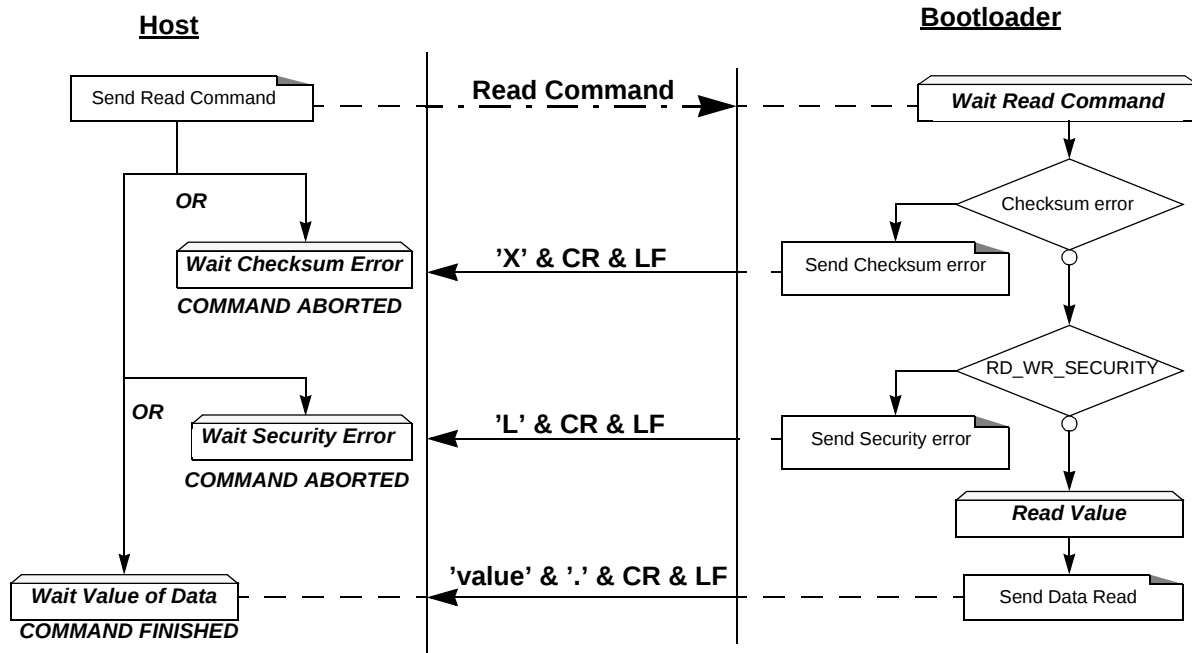
Figure 50. Read Flow
