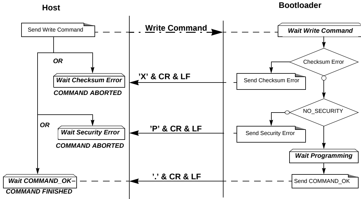
Figure 47. Write/Program Flow
