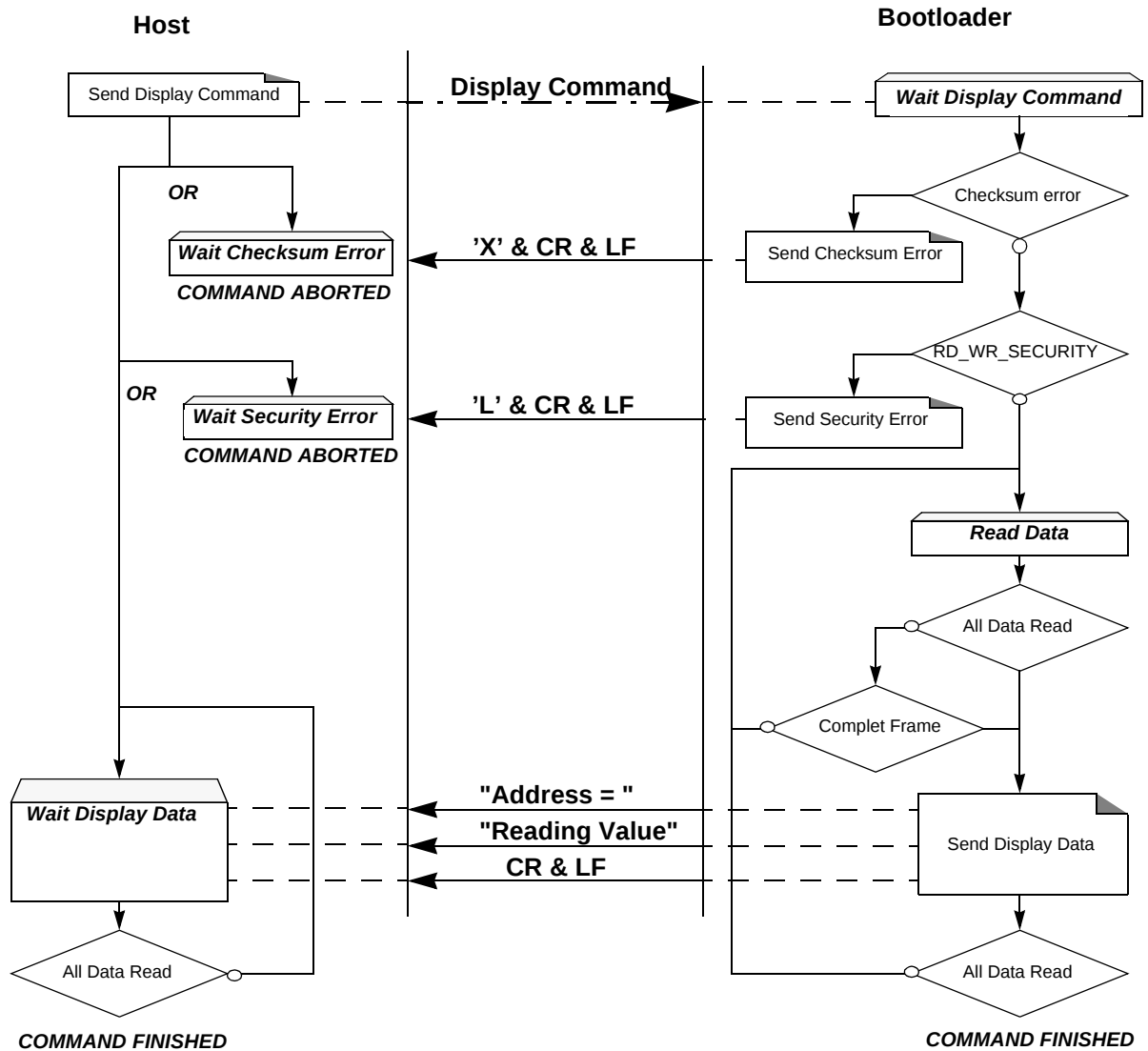
Figure 49. Display Flow
