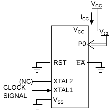
Figure 52. I_{CC} Test Condition, Idle Mode
