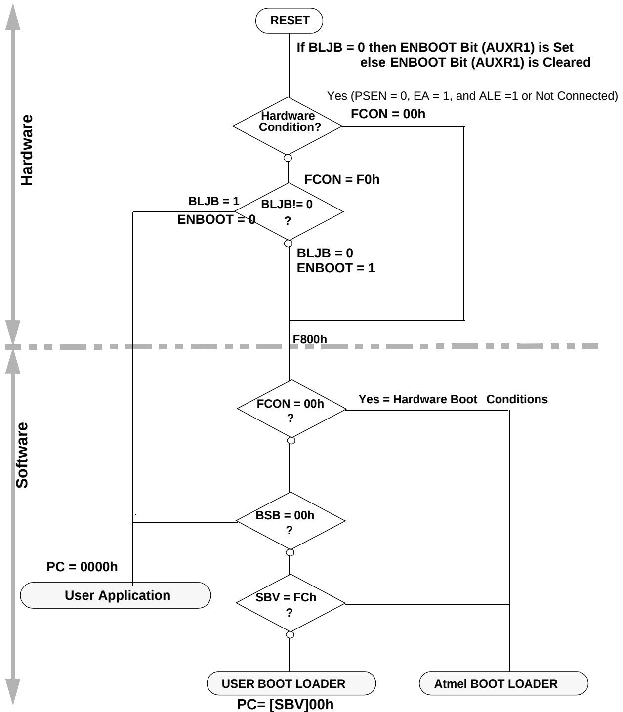
Figure 43. Bootloader Process
