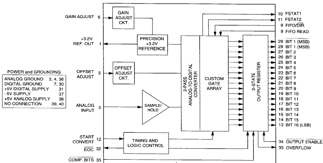
Figure 1. ADS-931 Functional Block Diagram
