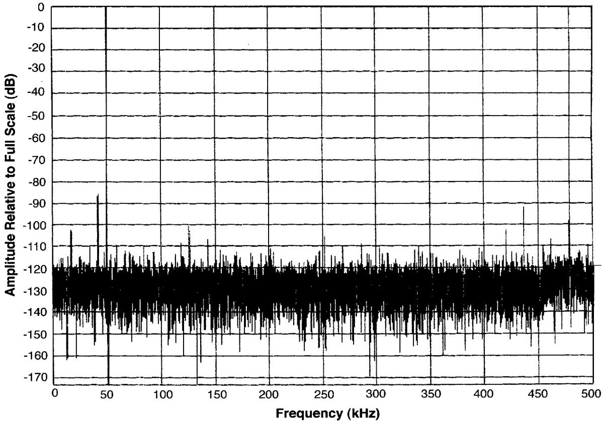
Figure 4. FFT Analysis of ADS-931 ( f_s = 1\text{MHz} , f_{in} = 485\text{kHz} , V_{in} = -0.5\text{dB} , 32,768-point FFT)
